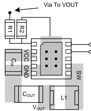
APW8805B Layout Consideration
