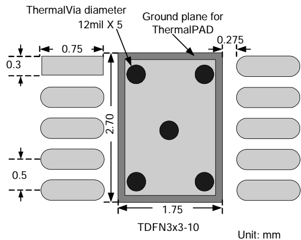
APW8805B Recommended Footprint
