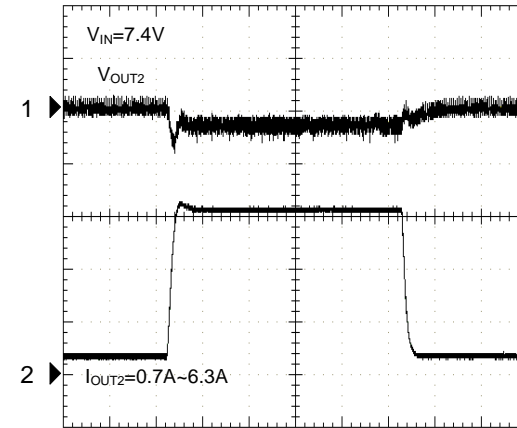
Load Transient
