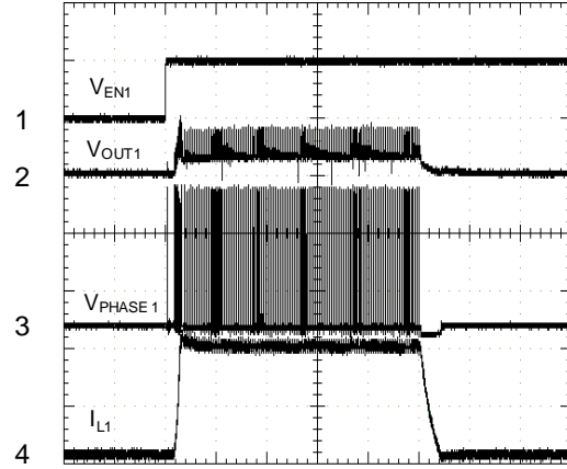
Current Limit, R_{LIM}=15k\Omega
