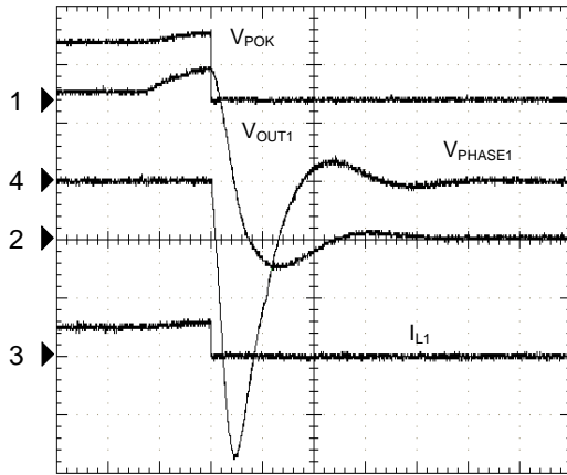
Over Voltage Protection
