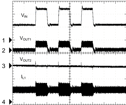
Line Transient
