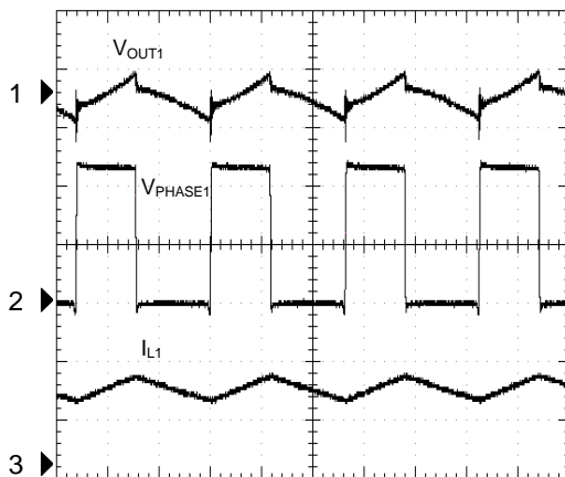
Output 1 Ripple Voltage
