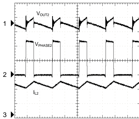
Output 2 Ripple Voltage
