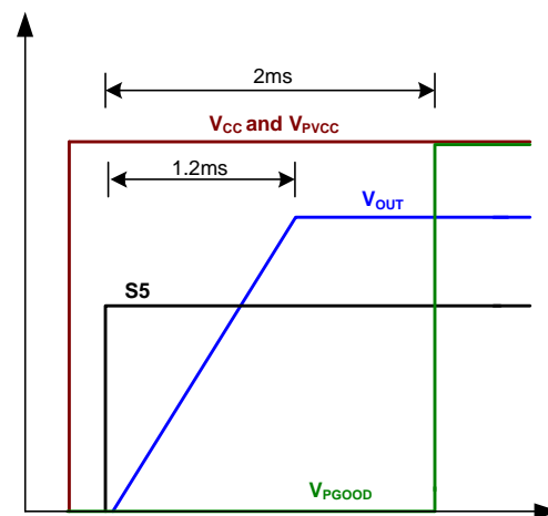
Fig1. Soft-Start Sequence
