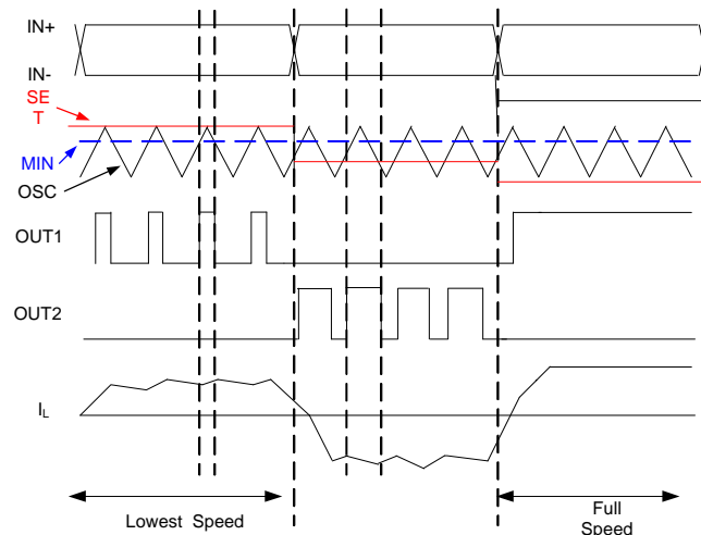
Figure 1. Rotation Waveform
