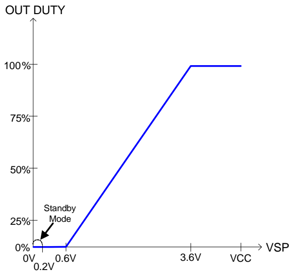
Figure 1: VSP Control
