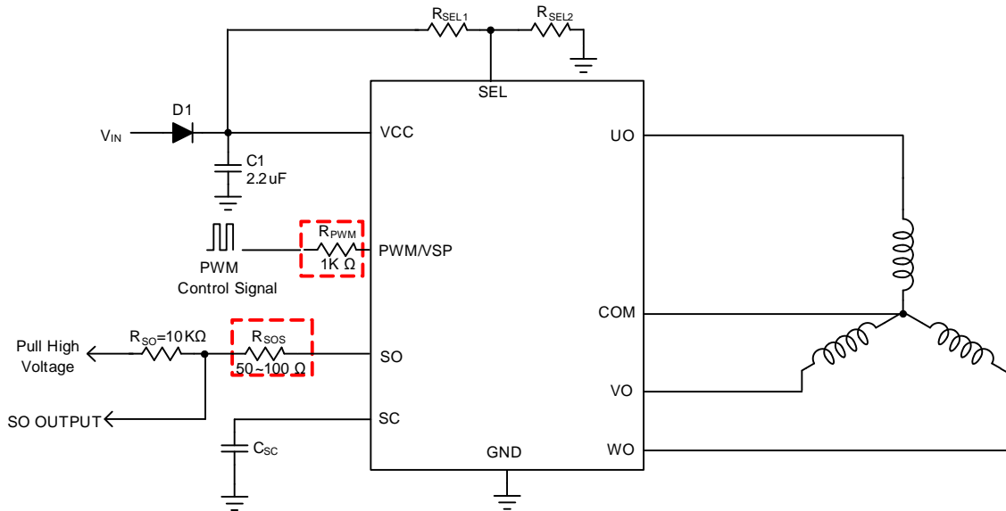
Circuit1: PWM Speed Control
