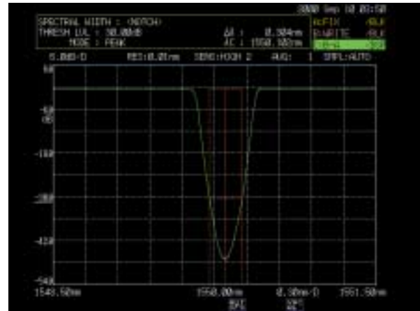
Measurement example of fiber grating notch width
