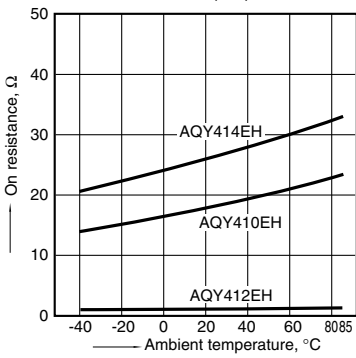
2. On resistance vs. ambient temperature characteristics
