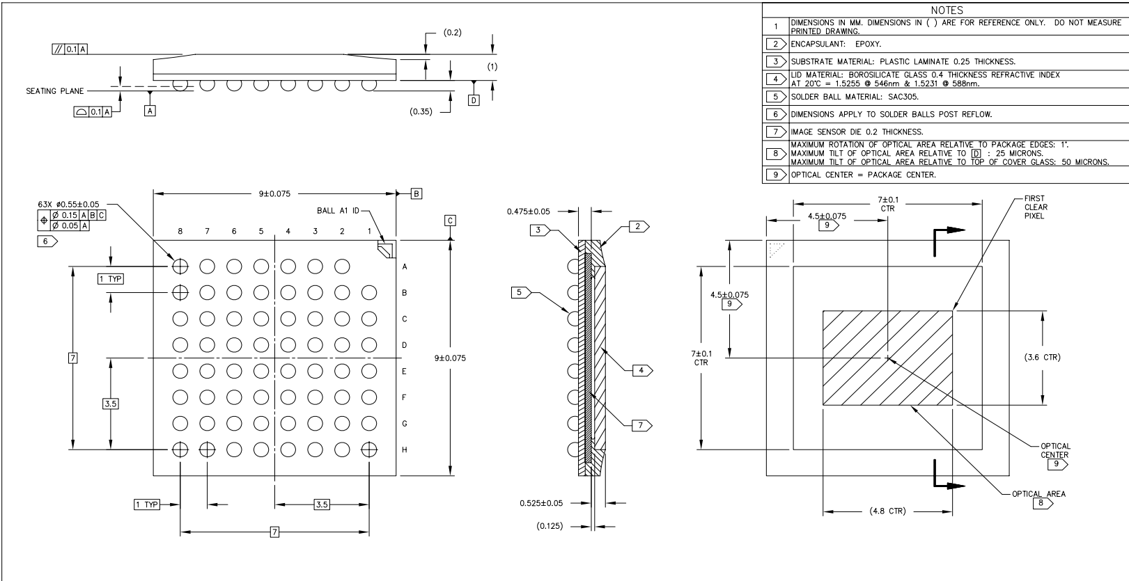
Figure 35: 64-Ball iBGA Package Outline Drawing
