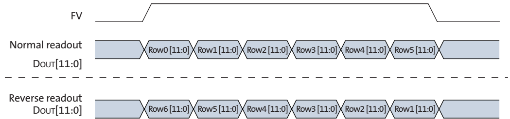
Figure 17: Six Rows in Normal and Row Mirror Readout Modes
