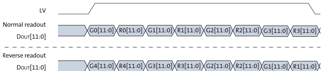
Figure 16: Six Pixels in Normal and Column Mirror Readout Modes
