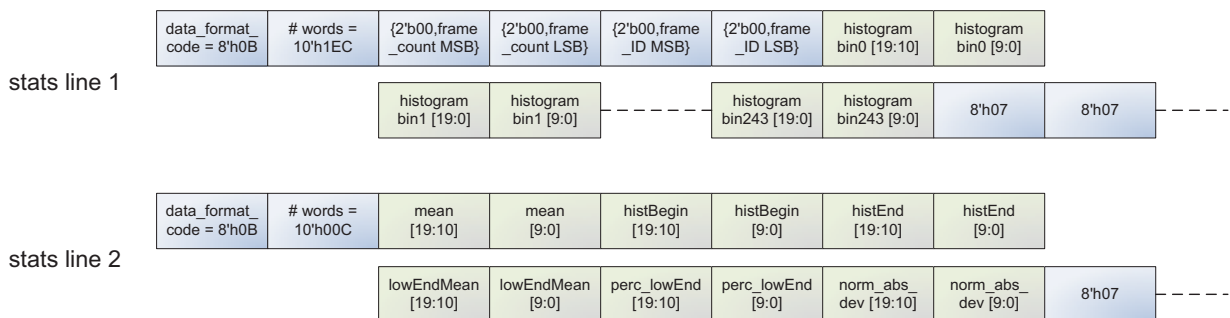
Figure 19: Format of Embedded Statistics Output within a Frame
