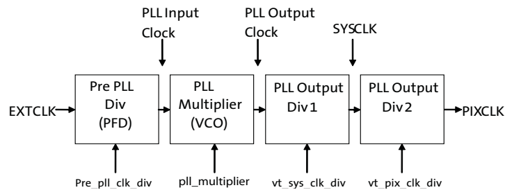
Figure 15: PLL-Generated Master Clock PLL Setup
