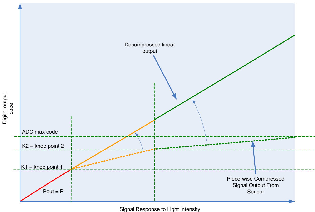
Figure 14: HDR Data Compression
