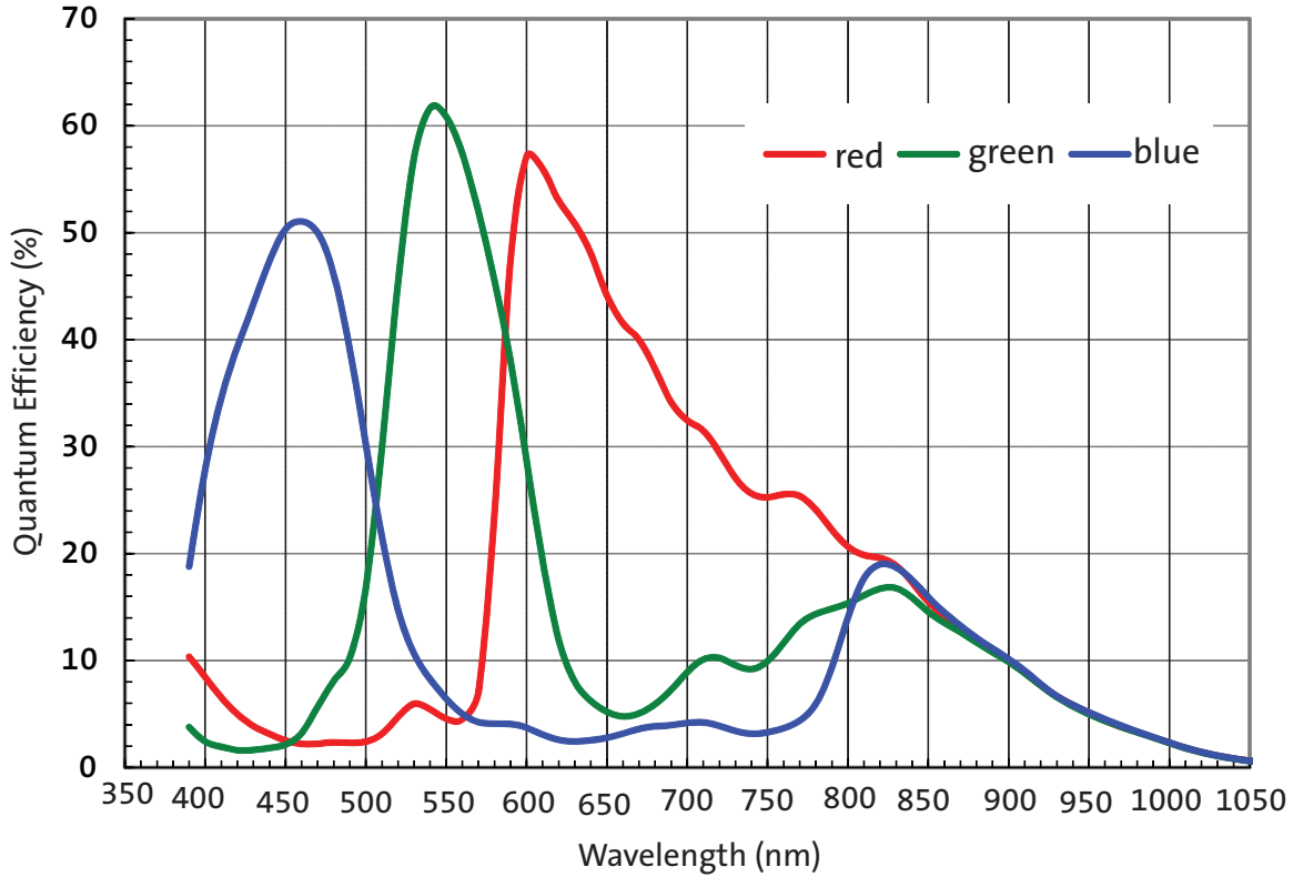
Figure 26: Quantum Efficiency – Color Sensor
