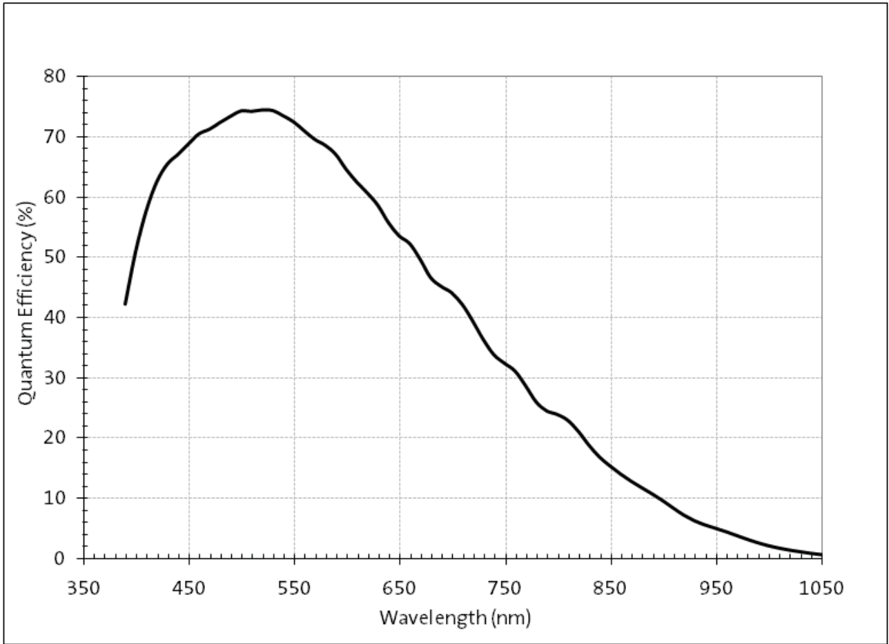
Figure 27: Estimated Quantum Efficiency – Monochrome Sensor
