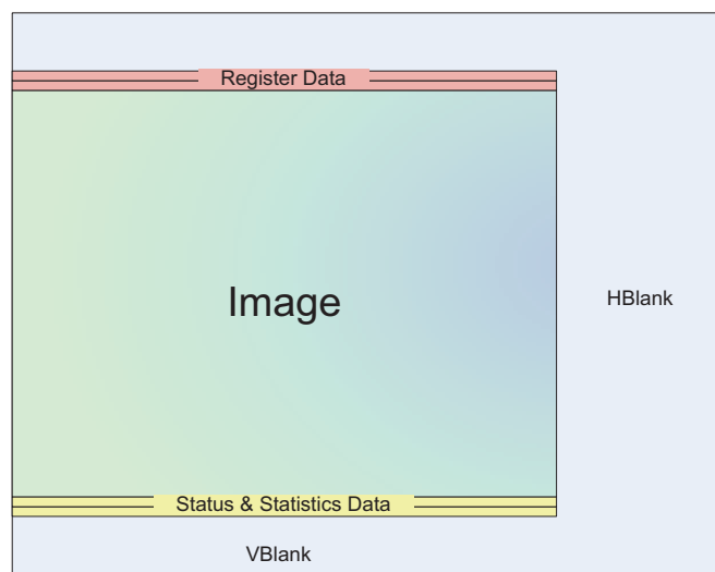
Figure 18: Frame Format with Embedded Data Lines Enabled
