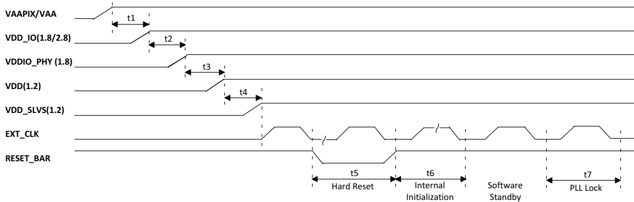
Figure 7. Power-Up Sequence
