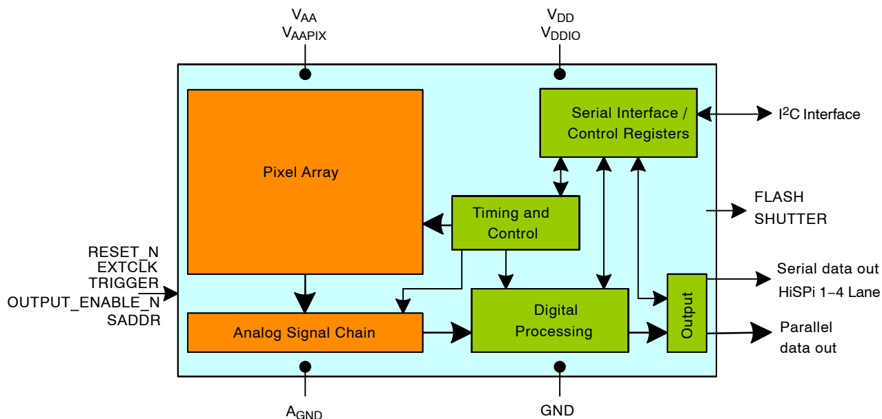
Figure 1. Block Diagram
