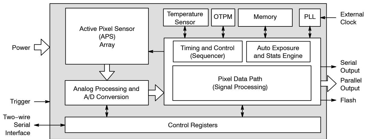
Figure 1. Block Diagram
