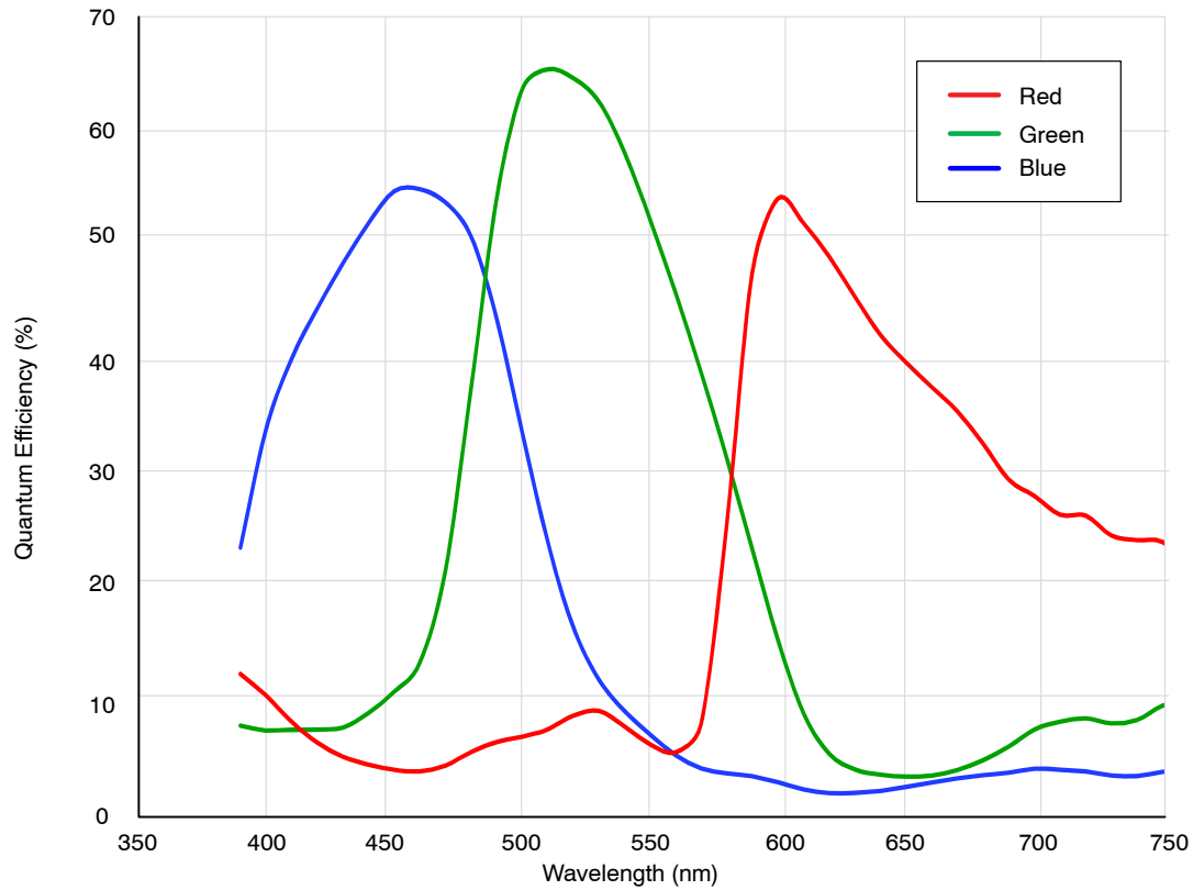
Figure 43. Quantum Efficiency
