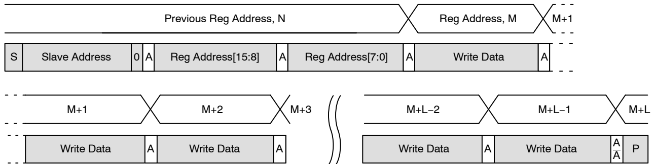
Figure 15. Sequential WRITE, Start at Random Location
