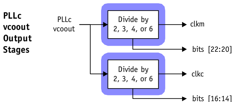
Figure 3-1. Ref_clk and PLLc vcoout Stages
