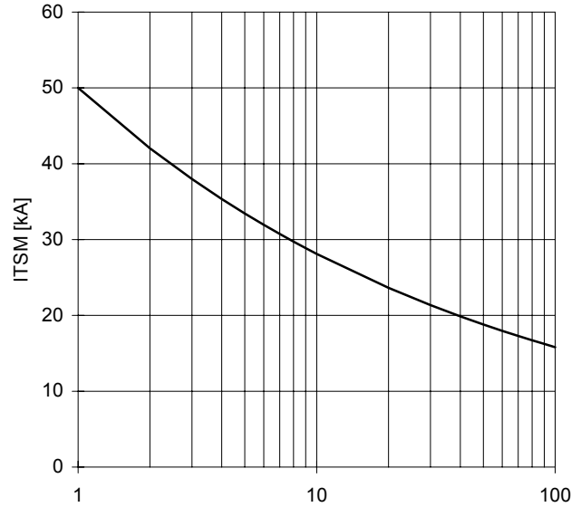
SURGE CHARACTERISTIC T_j = 150\text{ }^\circ\text{C}
