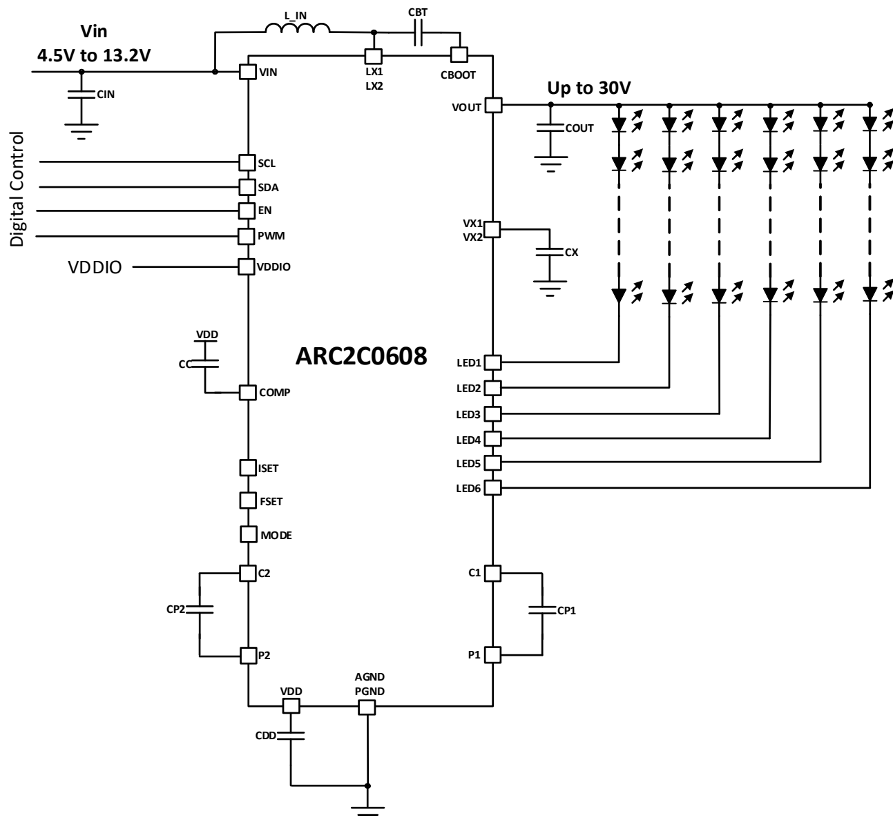
Figure 6. I²C Interface Application Schematic
