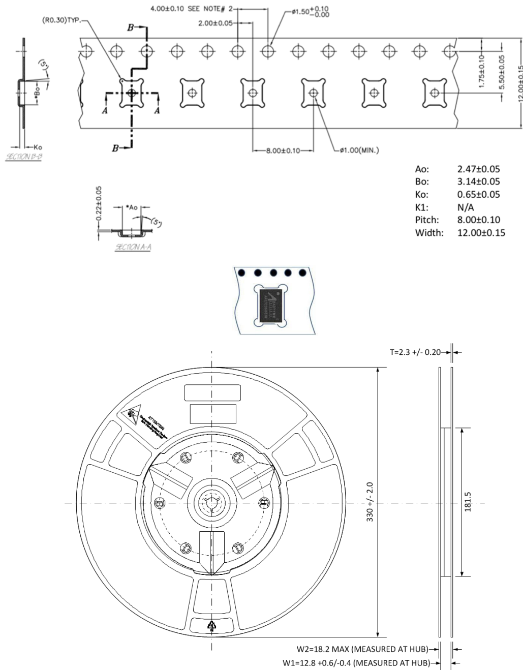
Figure 40. 2.985 mm × 2.315 mm WLCSP Tape and Reel Specification
