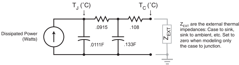
Figure 5b, TRANSIENT THERMAL IMPEDANCE MODEL
