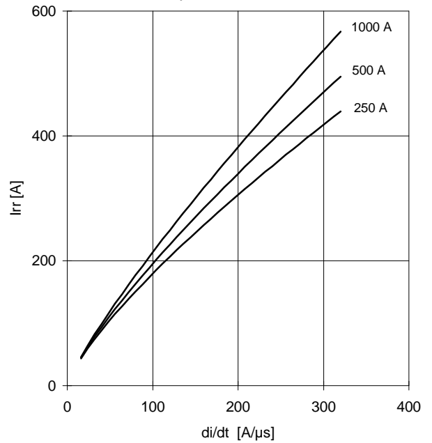
REVERSE RECOVERY CURRENT Tj = 150 °C
