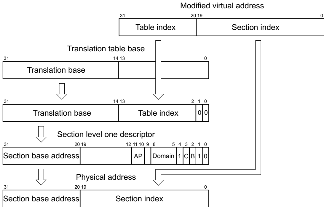
Figure 3-8 Section translation
