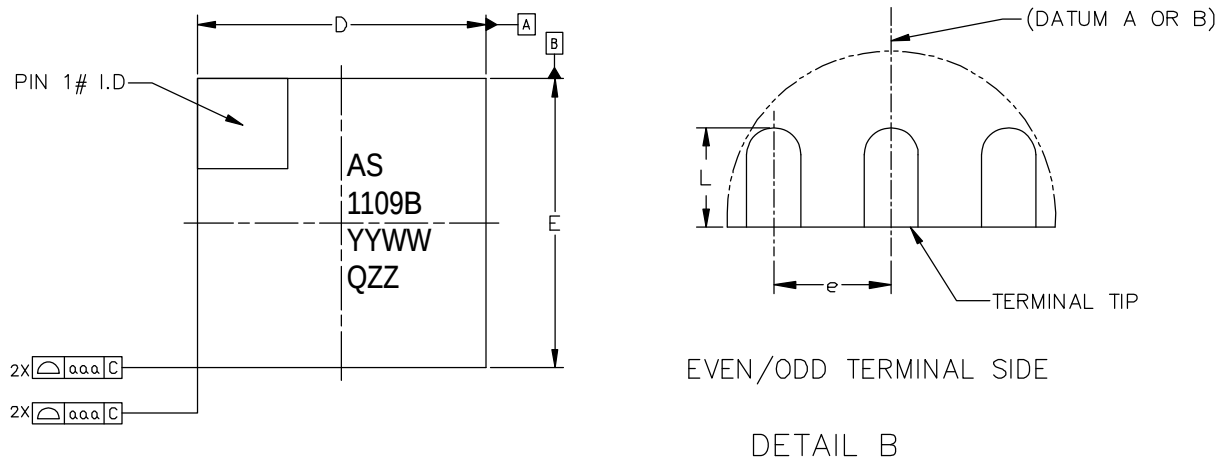
Figure 27. 16-pin QFN 4x4mm Package
