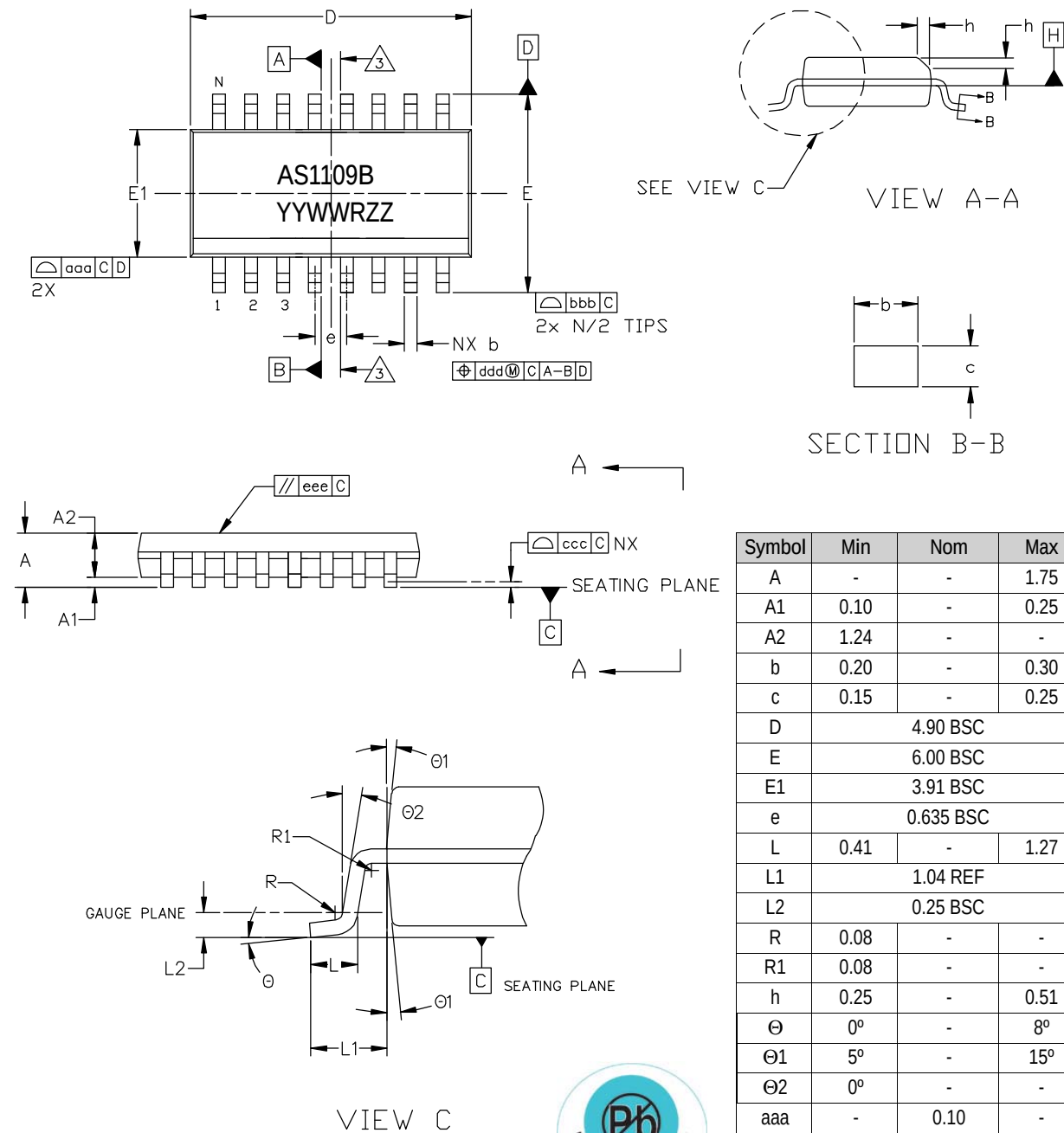
Figure 26. 16-pin QSOP-150 Package
