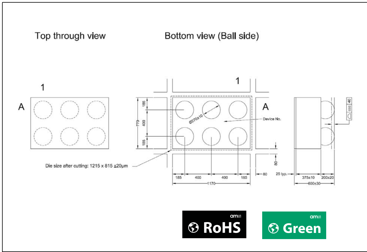
Figure 19: WL-CSP-6 0.4mm Pitch Package Drawing
