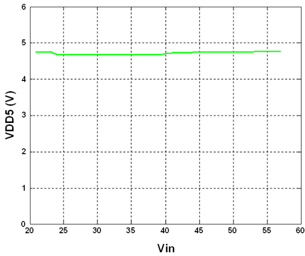
Figure 5 - VDD5 vs. V_{IN}
