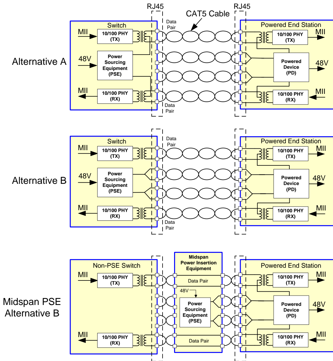
Figure 28 - IEEE® Std. 802.3af-2005 Power Feeding Schemes for 10/100 Systems
