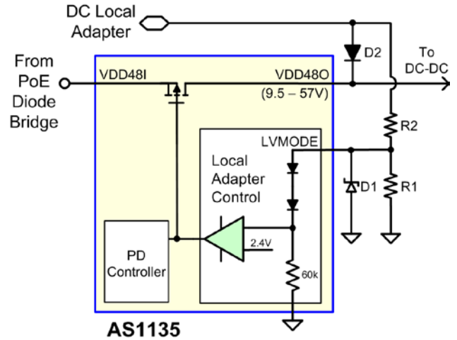
Figure 32 - LVMODE Implementation
