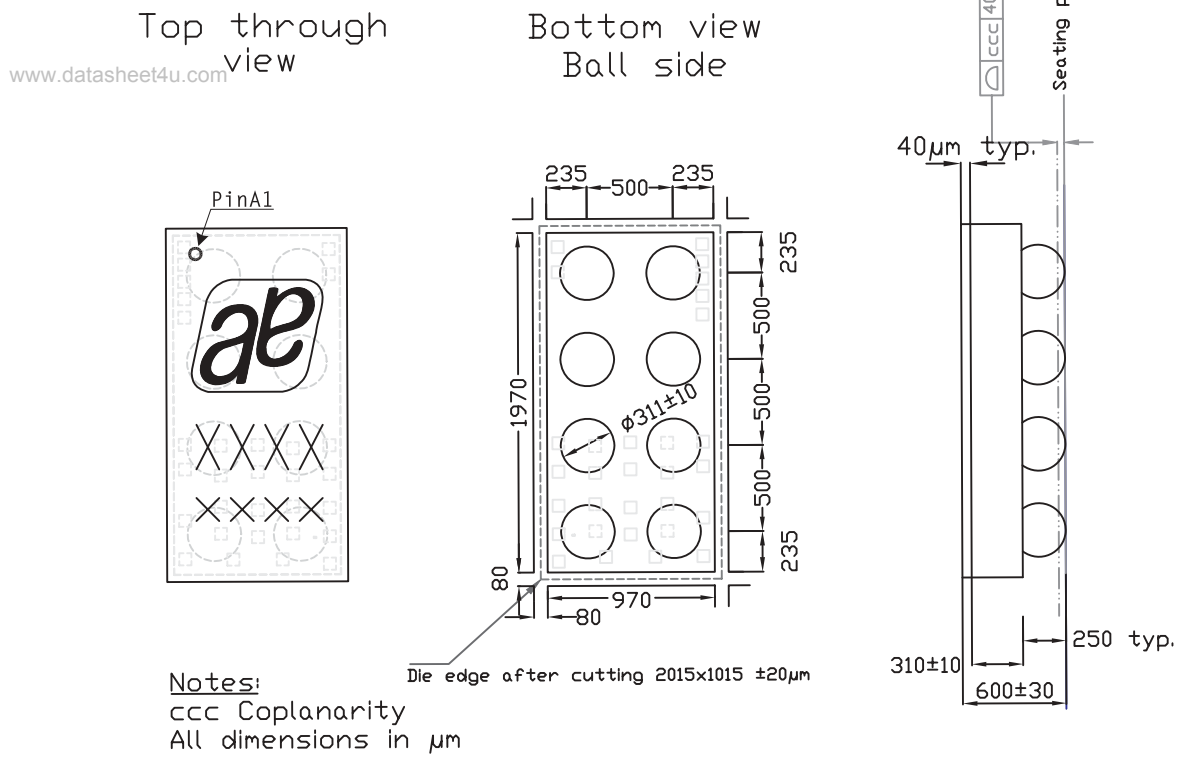
Figure 30. WL-CSP 8-bumps Package Diagram
