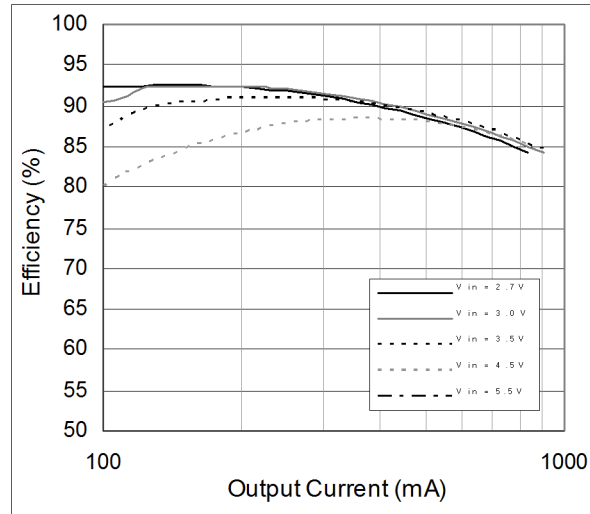
Figure 6. AS1346 Efficiency vs. V_{IN} , V_{OUT2} = 1.8V
