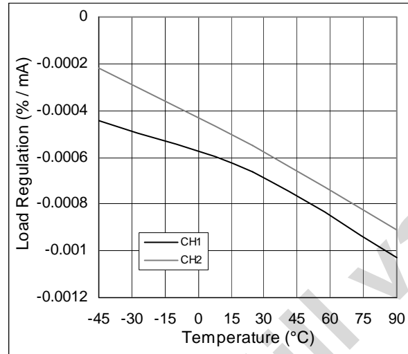
Figure 16. Load Regulation vs. Temperature
