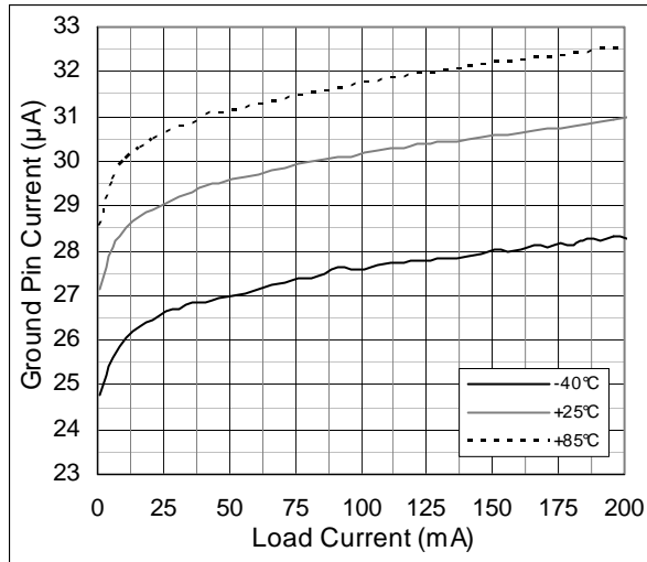
Figure 9. Ground Pin Current vs. Load Current
