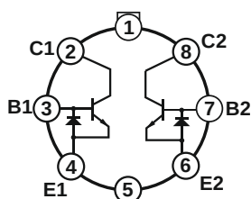
AS194H, AS394H, AS394CH Metal Can Package (TO5-8)
