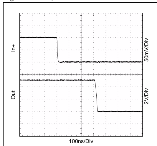
Figure 16. t_{PD-} ; V_{OD} = 50mV
