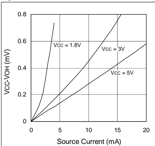
Figure 8. V_{OH} vs. I_{SOURCE}
