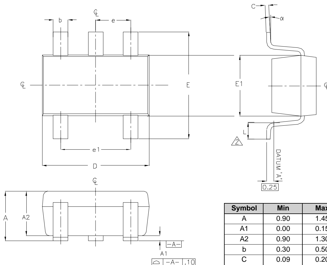
Figure 31. 5-pin SOT23 Package
