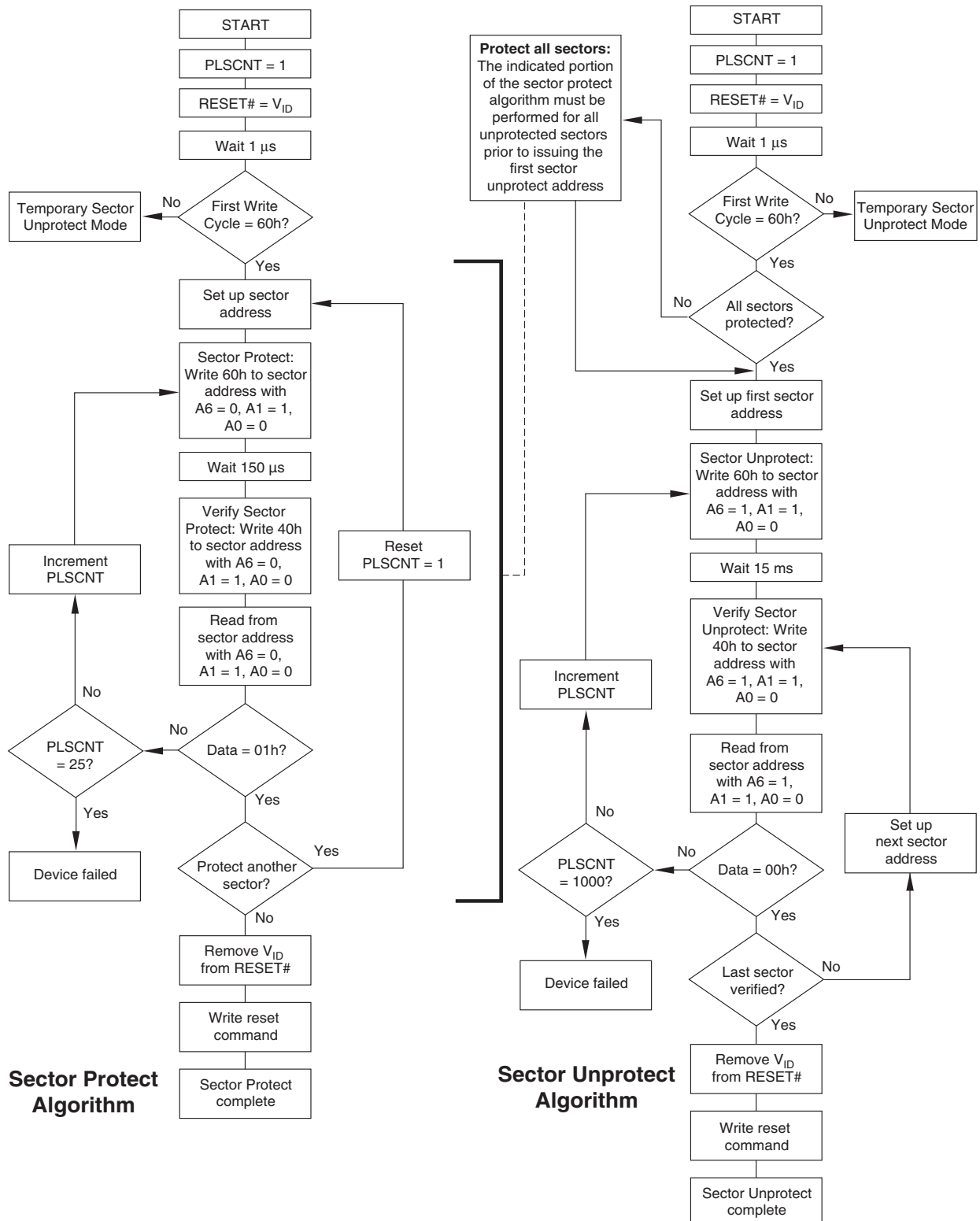
Figure 2. In-System Sector Protect/Unprotect Algorithms
