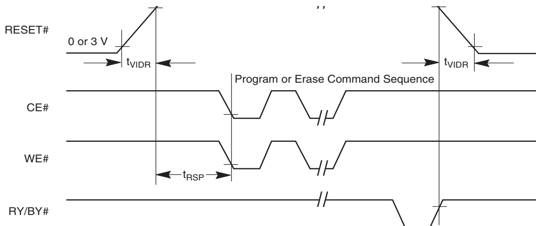
Figure 21. Temporary Sector Unprotect/Timing Diagram
