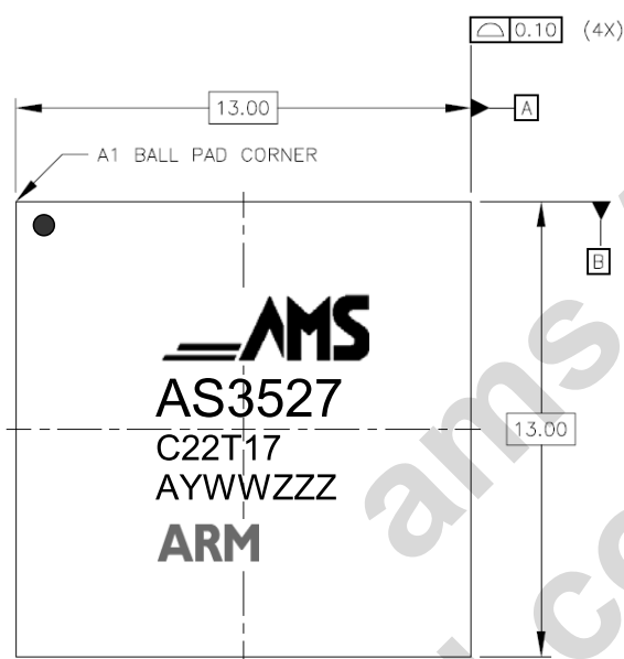
Figure 69 CTBGA224 Package Marking
