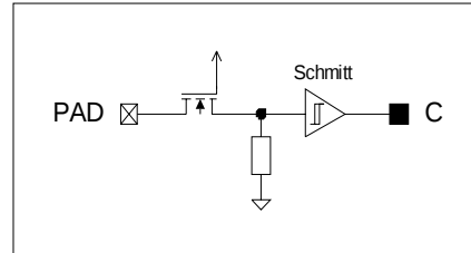
Figure 73 Digital Input with Schmitt Trigger and Pull-Down
