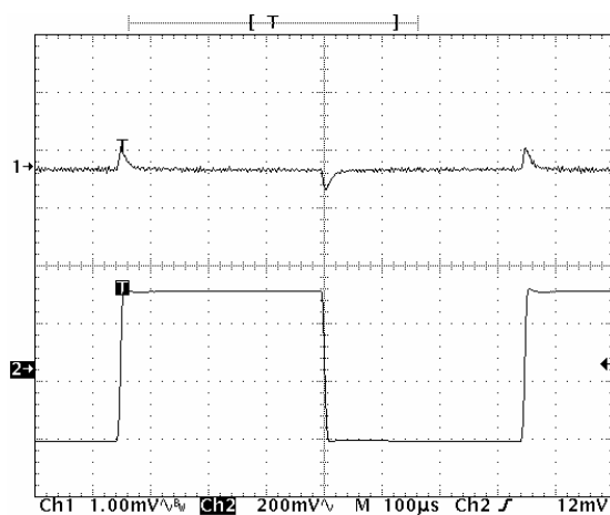
Load Regulation
