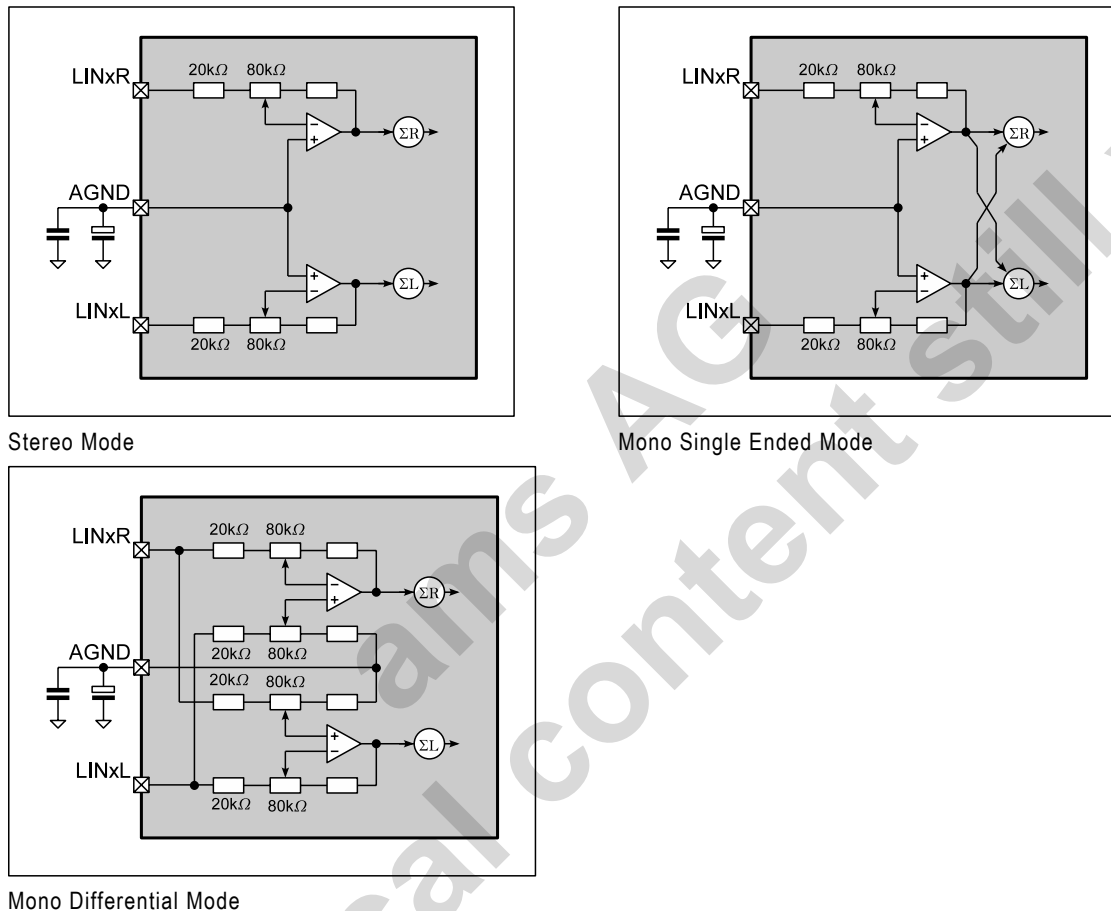
Figure 42 Line Inputs
