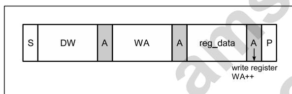
Figure 50 Page Write
