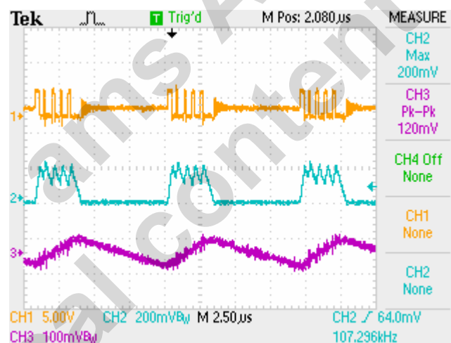
Figure 59 –DCDC buck with enabled current force / pulse skip mode
