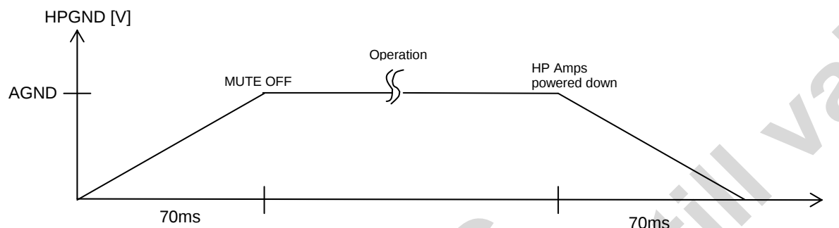
Figure 46 HP POP-Click Suppression
