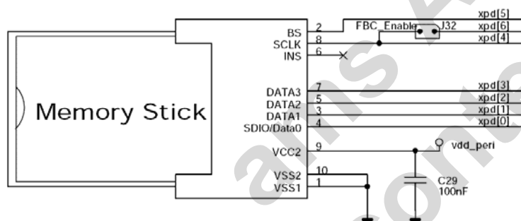
Figure 13 external memory stick connection
