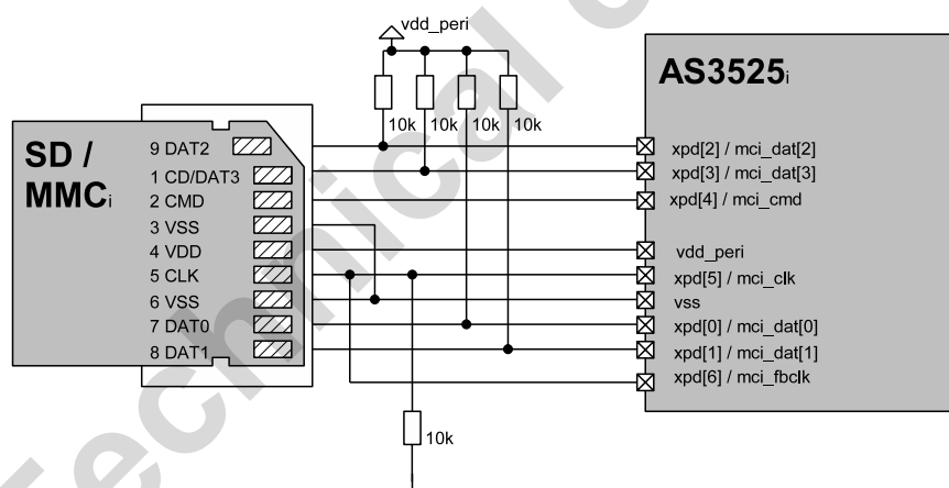
Figure 20 Connecting SD / MC to GPIO-D
