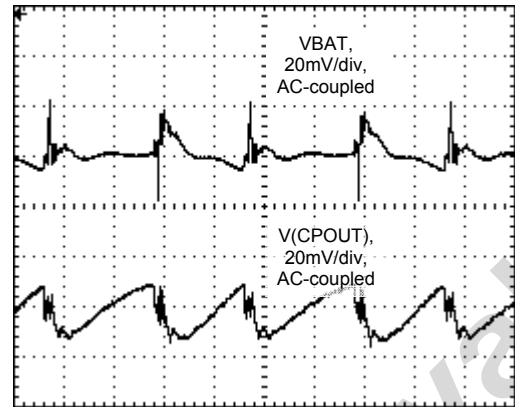
Figure 10 – Charge Pump Input and Output Ripple 1:2 Mode, 100mA load
