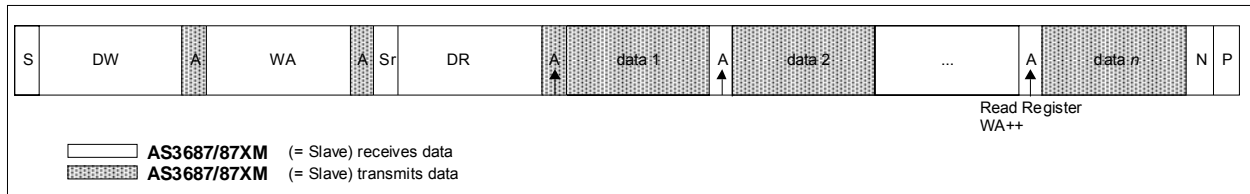
Figure 40 – Serial Interface Sequential Read
