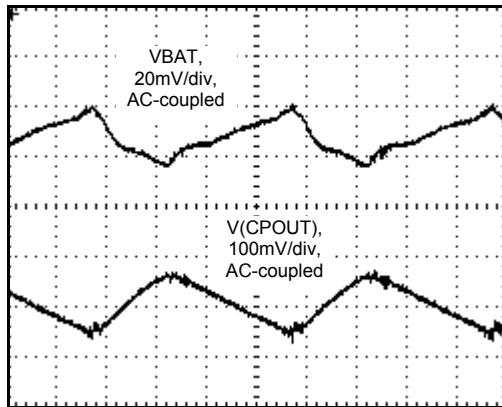
Figure 9 – Charge Pump Input and Output Ripple 1:1.5 Mode, 100mA load
