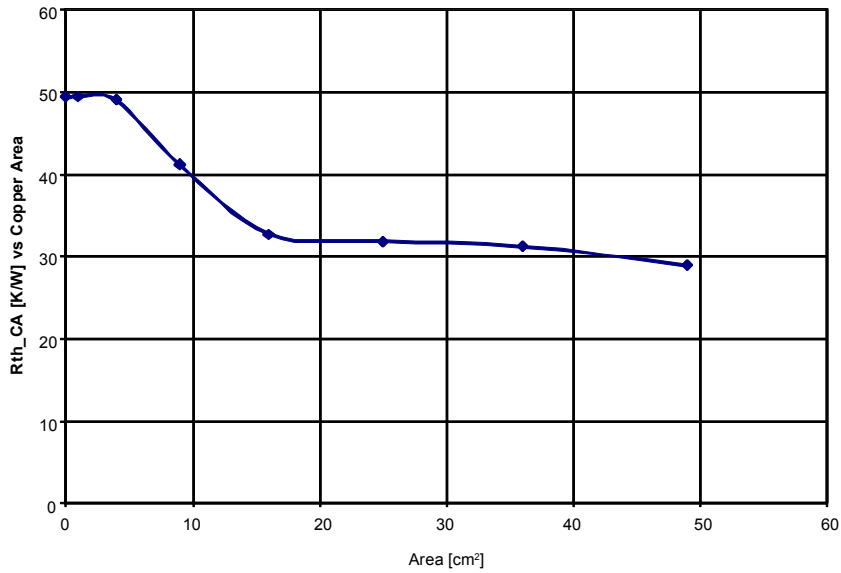
Figure 8.33 : Rth_CA [°C/W] vs Copper Area
