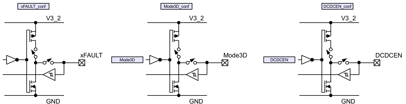
Figure 8.16 : GPIO
