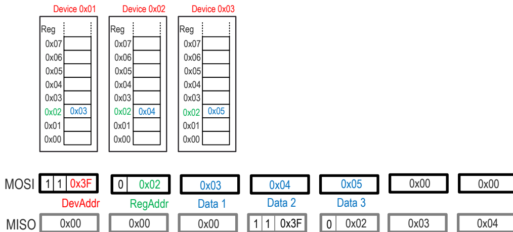
Figure 8.24 : Write to Reg0x02 of Dev0x01 – Dev0x03
