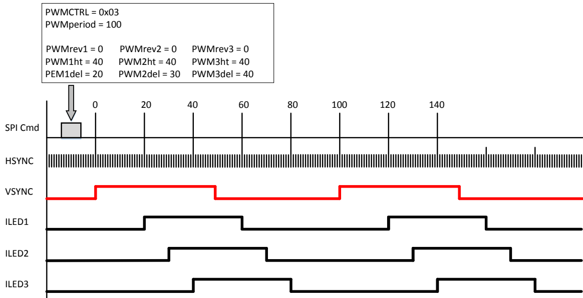
Figure 8.9 : PWM Example 1
