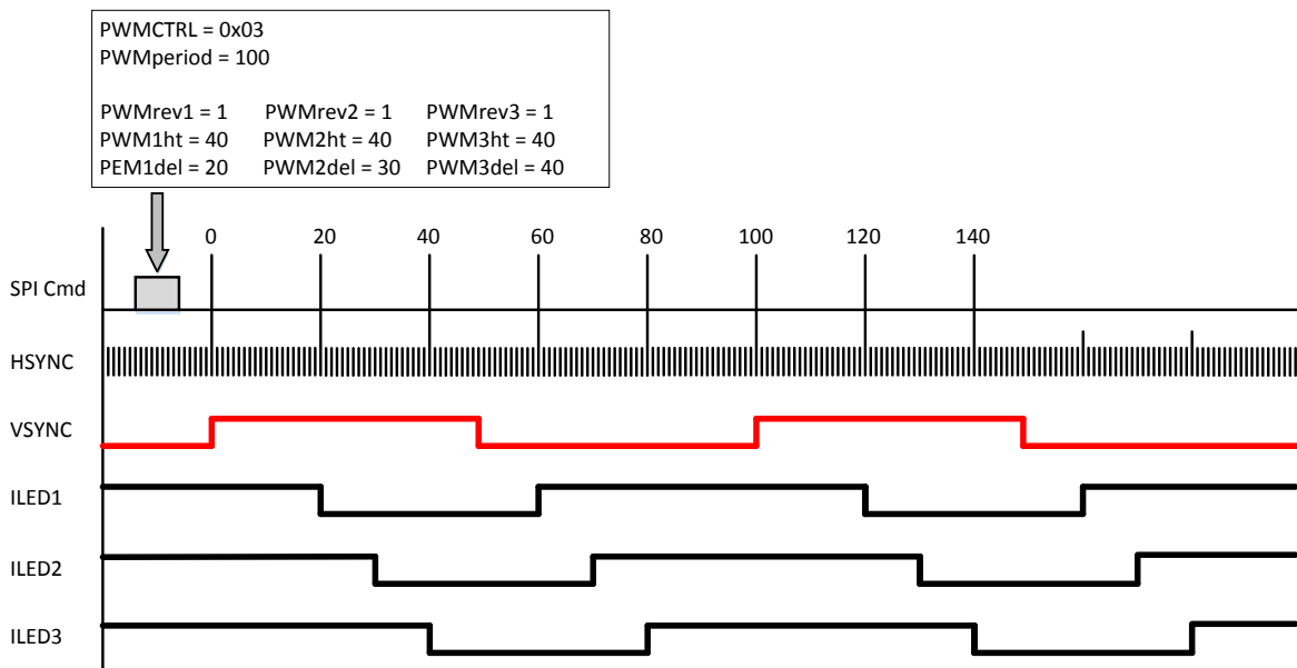
Figure 8.10 : PWM Example 2
