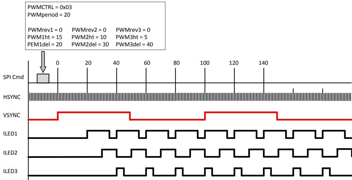
Figure 8.11 : PWM Example 3
