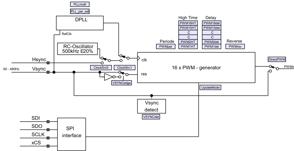
Figure 8.5 : PWM Generators
