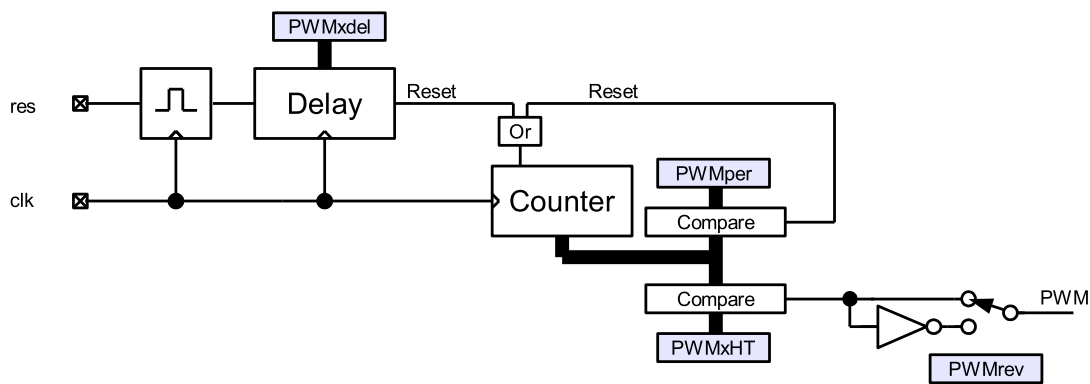
Figure 8.6 : PWM Counter
