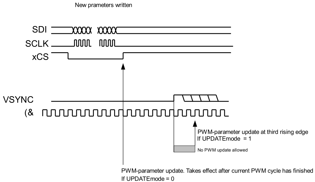
Figure 8.8 : UPDATE mode
