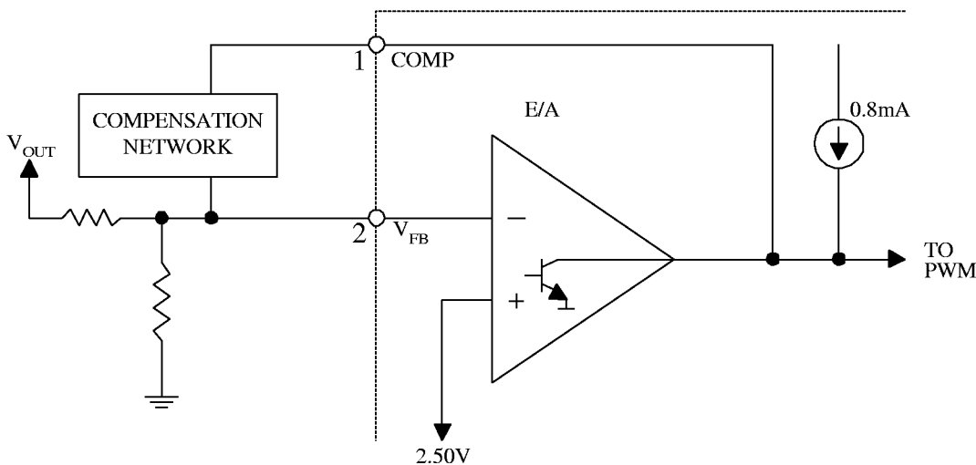
Figure 17. Error Amplifier Compensation
