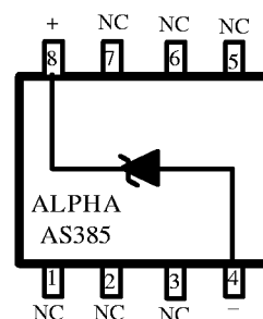
8-Pin Surface Mount
