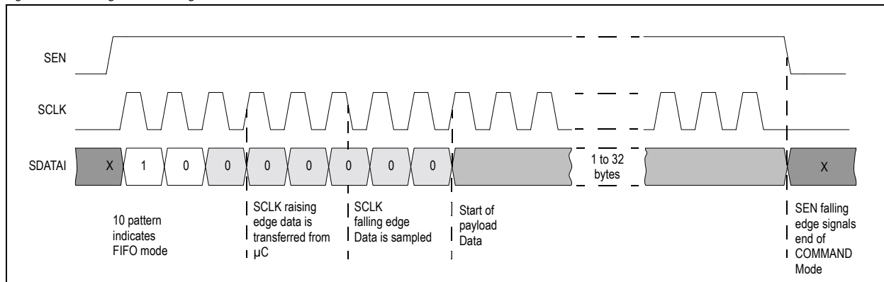
Figure 9. Loading Transmitting Data into FIFO
