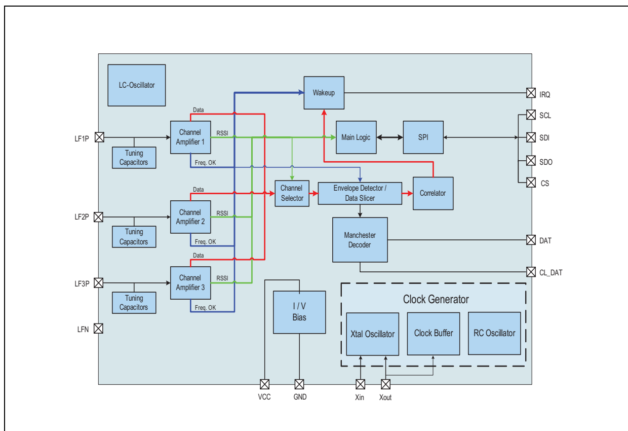
Figure 19: Block Diagram of LF Wake-Up Receiver AS3933
