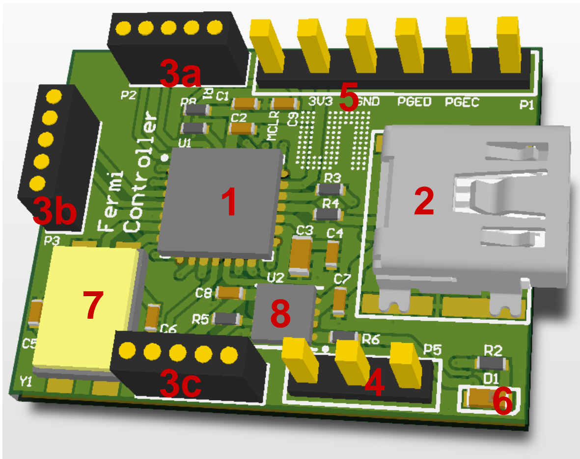
Figure 2 - Controller Part
