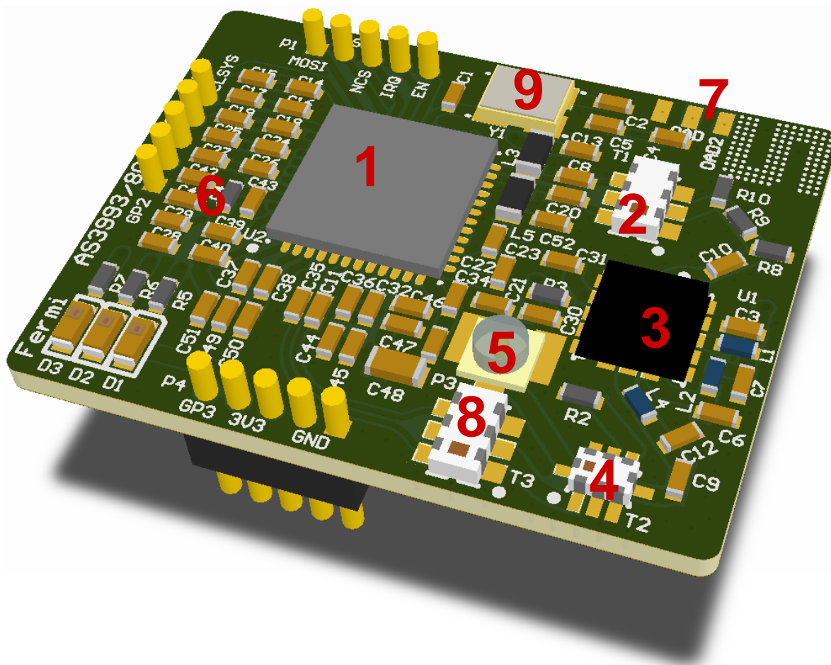
Figure 1 - Reader Part
