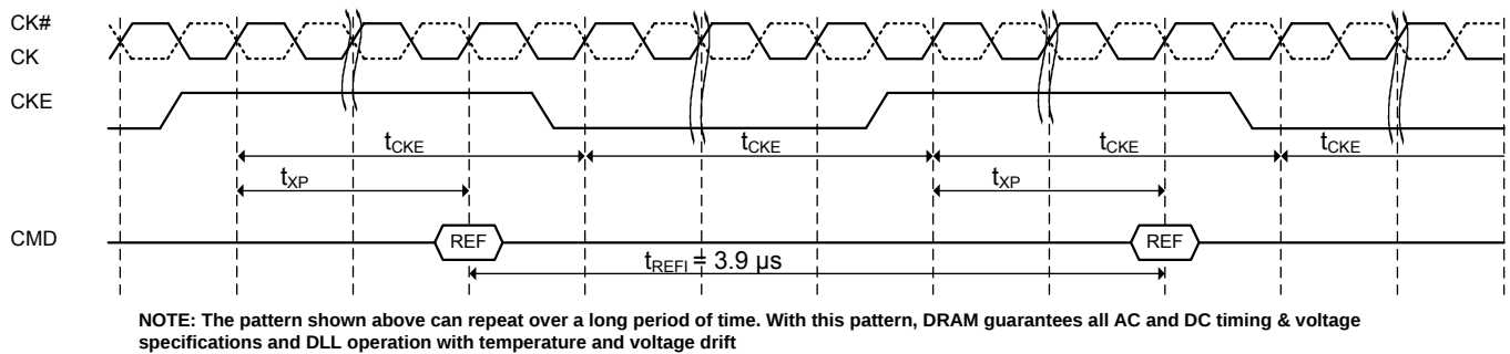
Figure 37.2.CKE intensive environment
