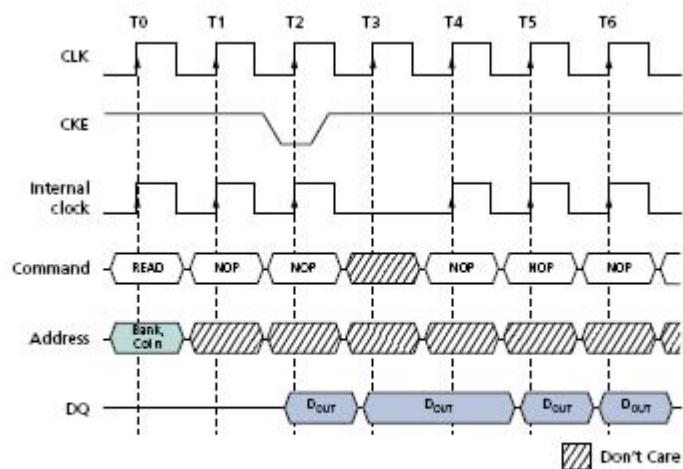
Figure 49: Clock Suspend During READ Burst
