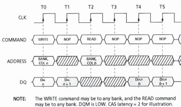
FIGURE 16: Random WRITE Cycles
