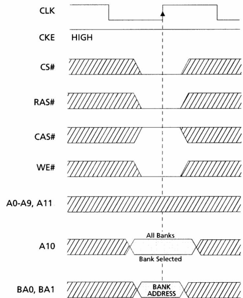
FIGURE 20: PRECHARGE Command
