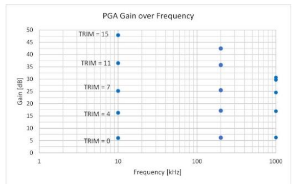
Figure 44: PGA Gain in [dB] vs. Frequency at 22°C
