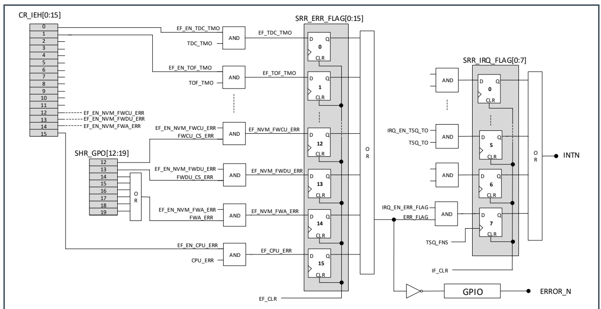
Figure 75: Hardware Error Flags
