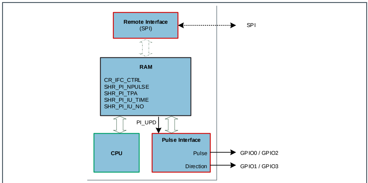
Figure 94: Pulse Interface: Functional Blocks and Variables
