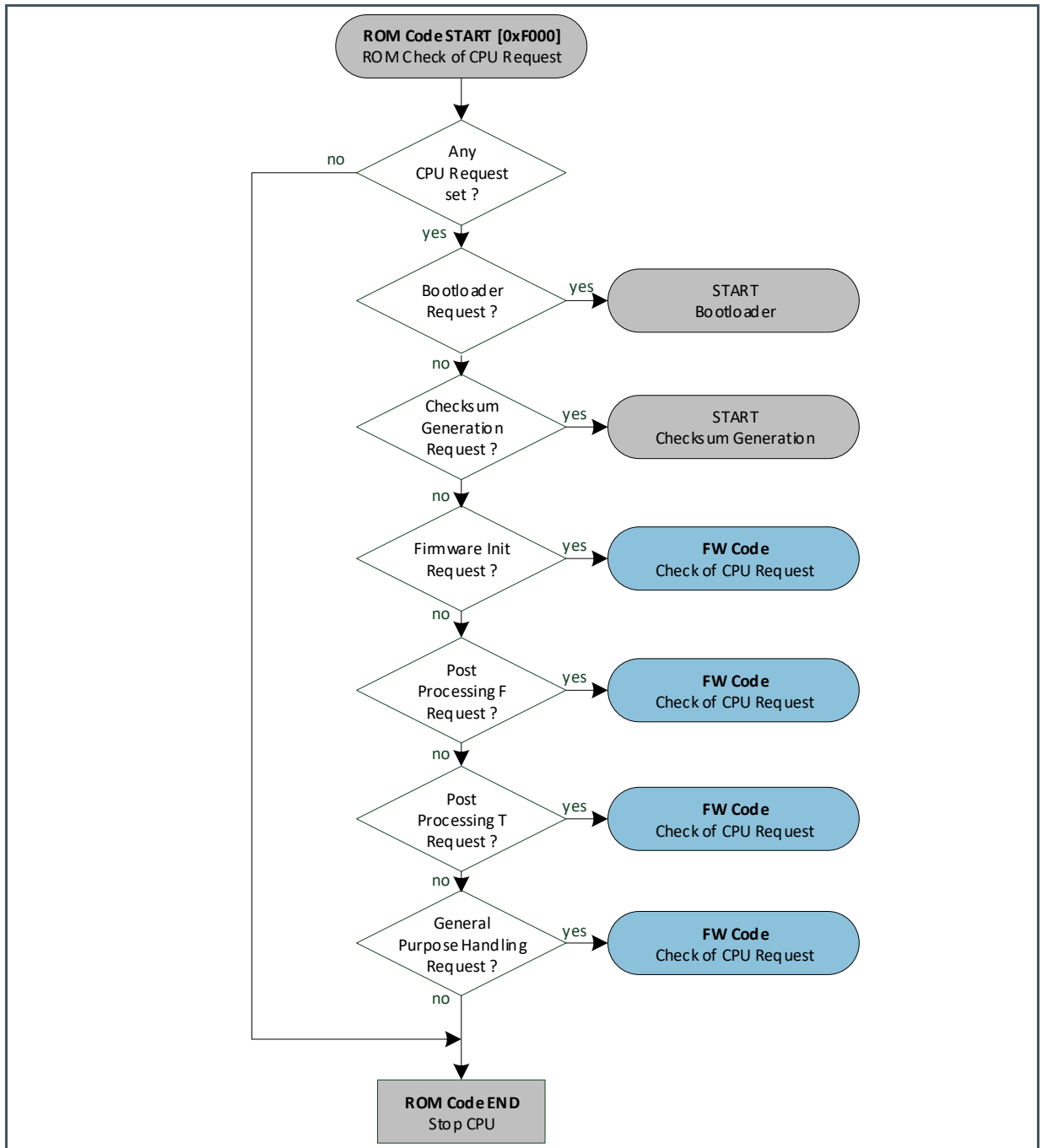
Figure 102: CPU Request Handling
