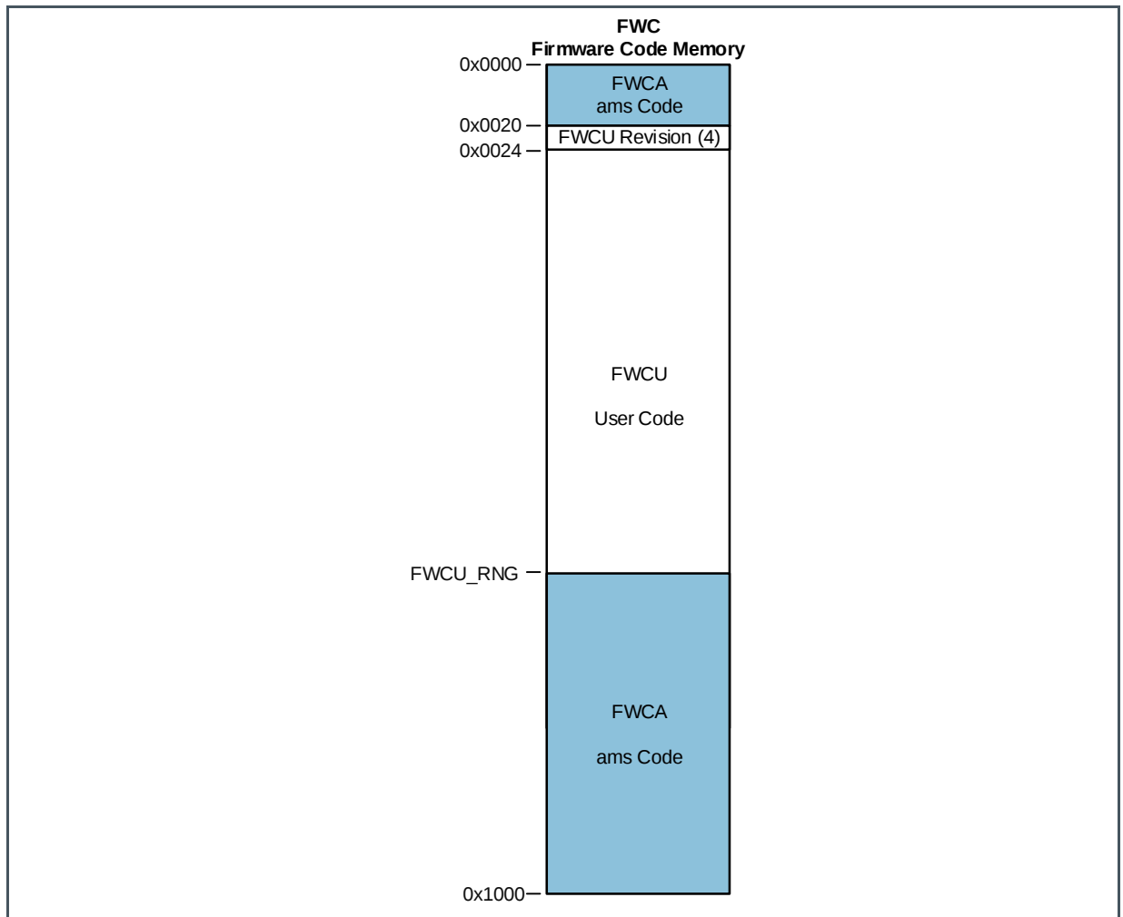
Figure 109: Program Area
