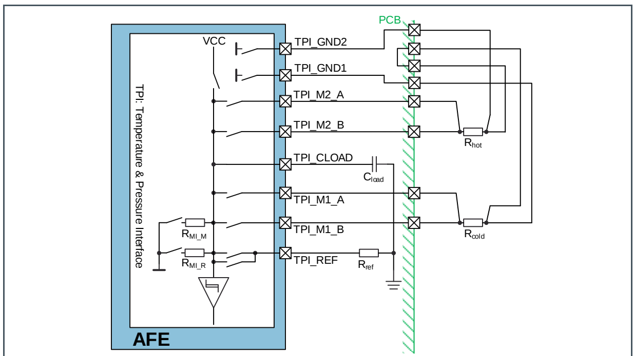
Figure 65: Temperature sensor, 4-wire connection
