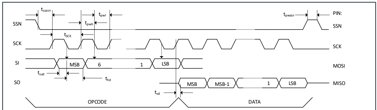
Figure 17: SPI Read
