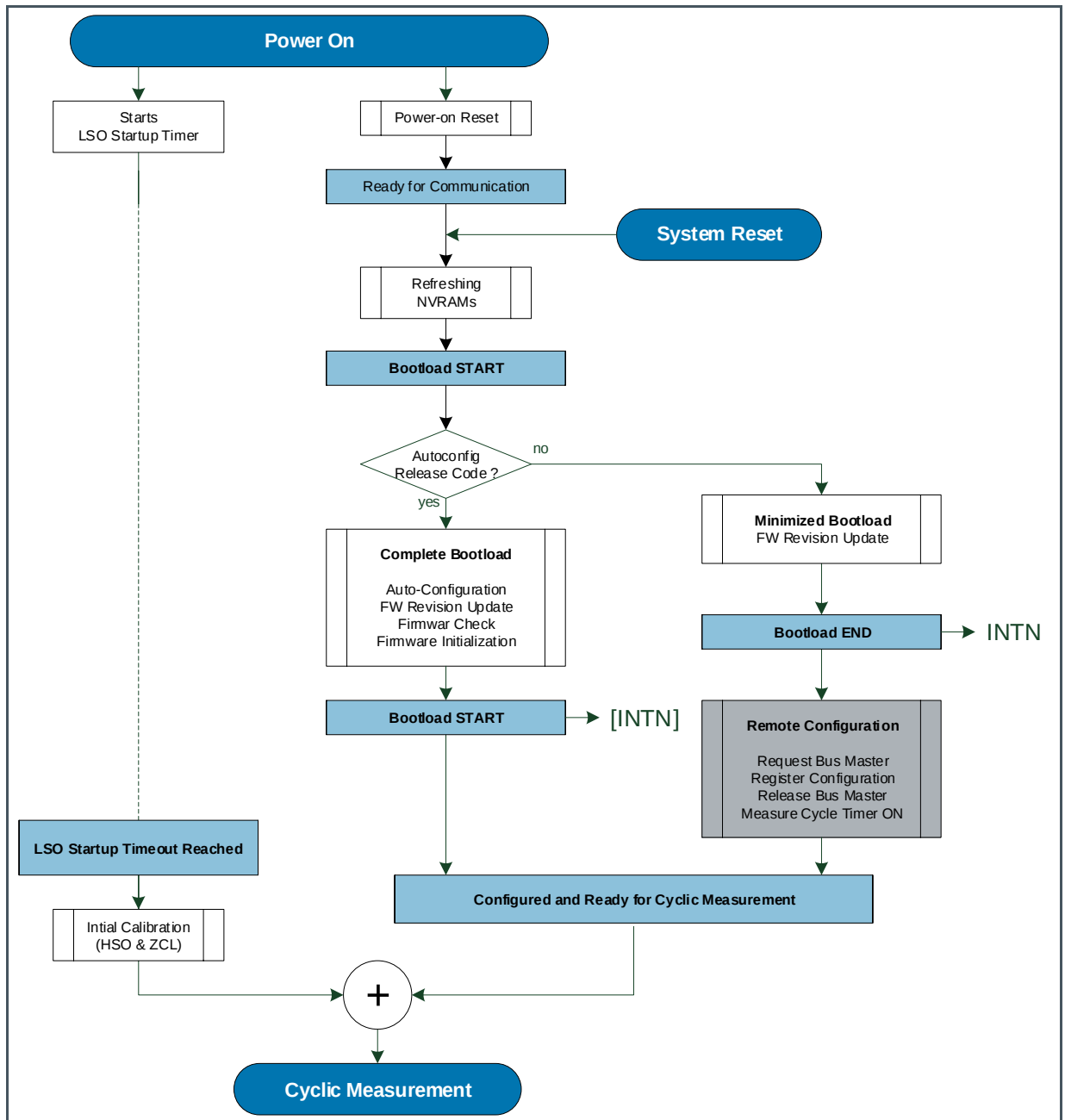
Figure 41: Start / Restart Sequence
