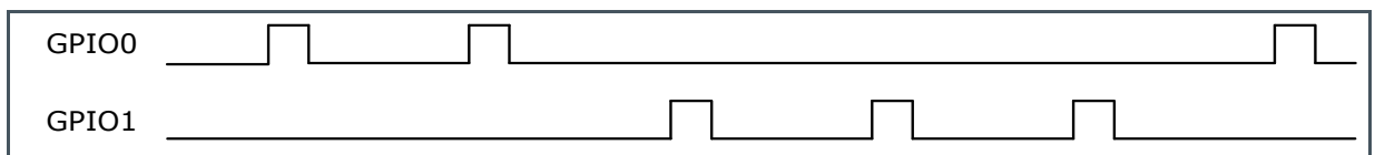
Figure 96: PI_OUT_MODE = 1
