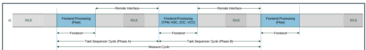
Figure 36: 2-phase Mode
