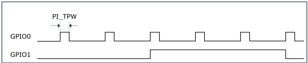
Figure 95: PI_OUT_MODE = 0
