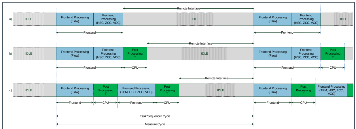
Figure 35: 1-phase Mode
