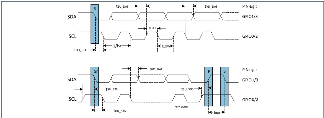
Figure 19: 2-wire Master Interface Timing
