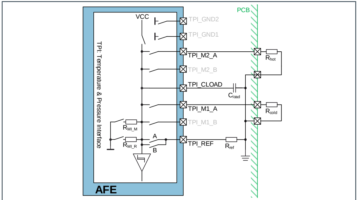
Figure 63: Temperature sensor, 2-wire connection
