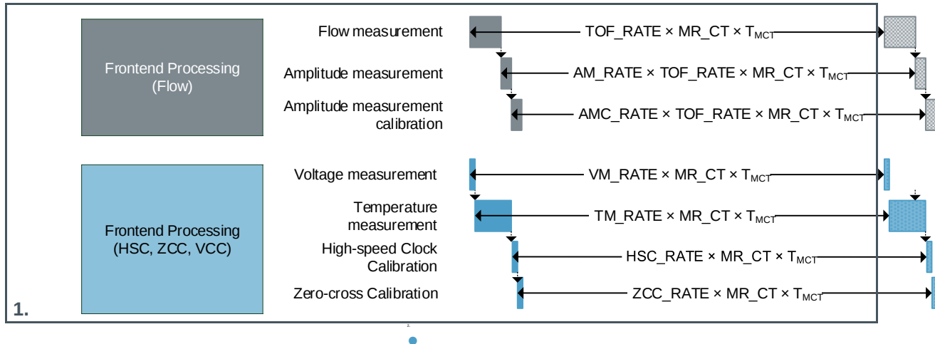
Figure 32: Individual Task Rates
