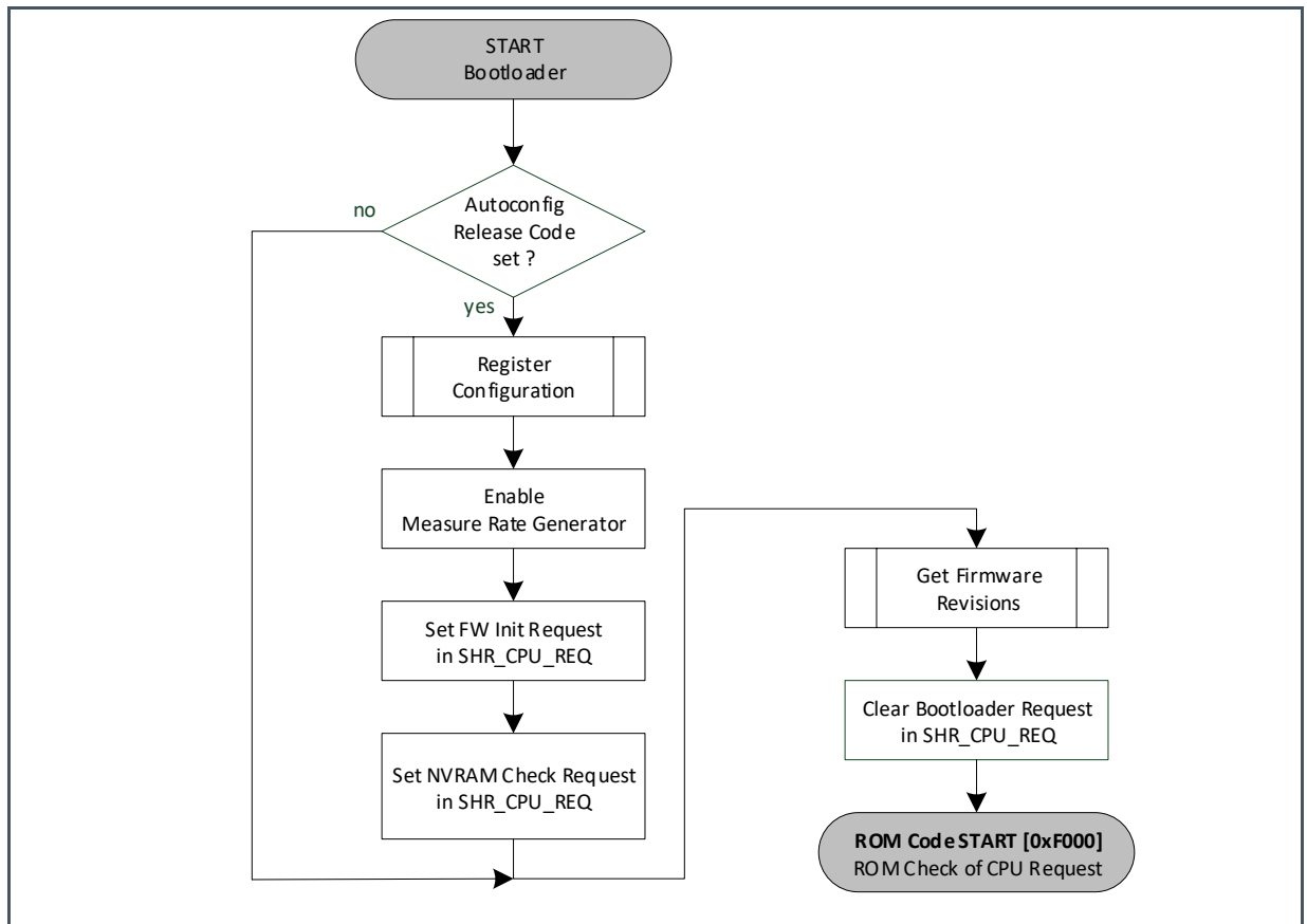
Figure 103: Bootloader actions
