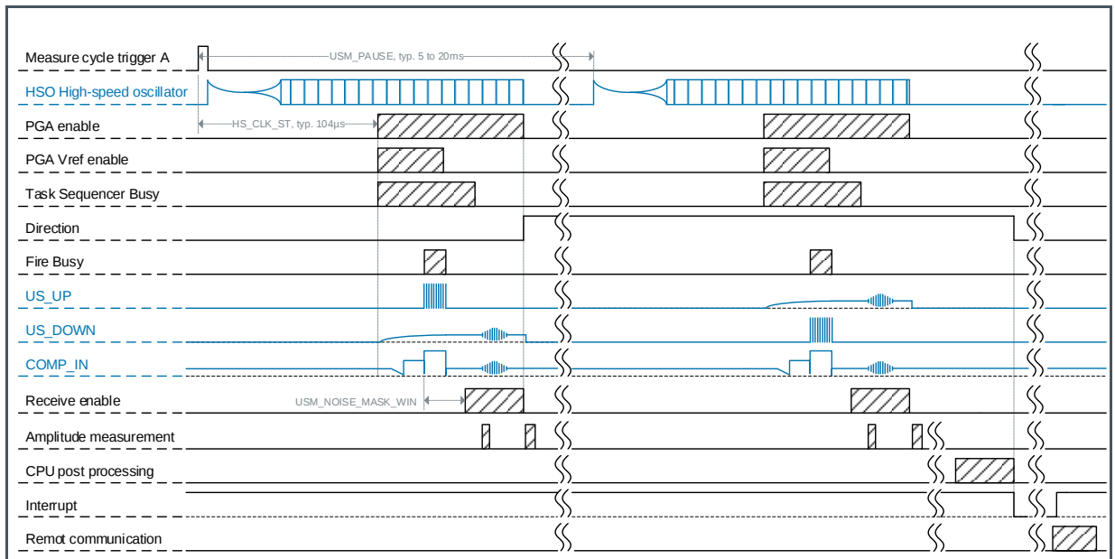
Figure 48: Timing Diagram Flow Measurement
