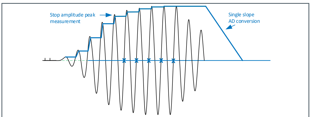
Figure 60: Amplitude Measurement
