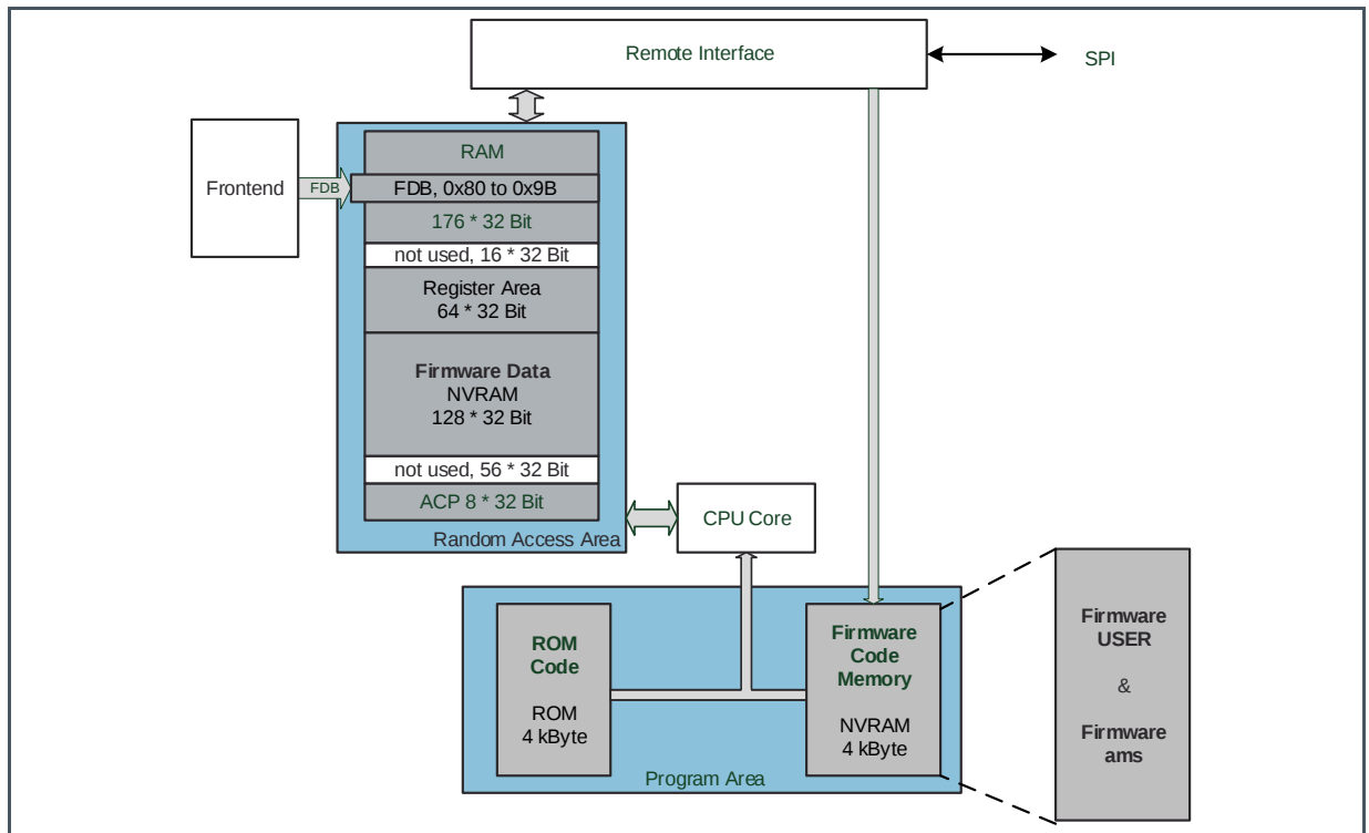
Figure 108: Memory Organization
