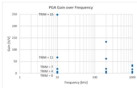
Figure 43: PGA Gain in [V/V] vs. Frequency at 22°C
