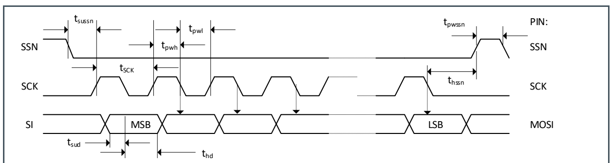
Figure 16: SPI Write
