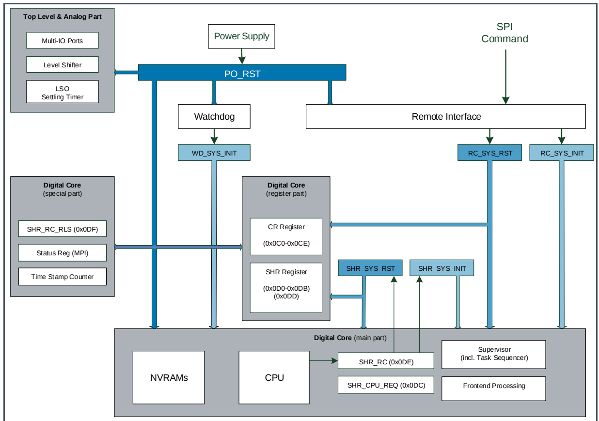
Figure 26: Reset Distribution
