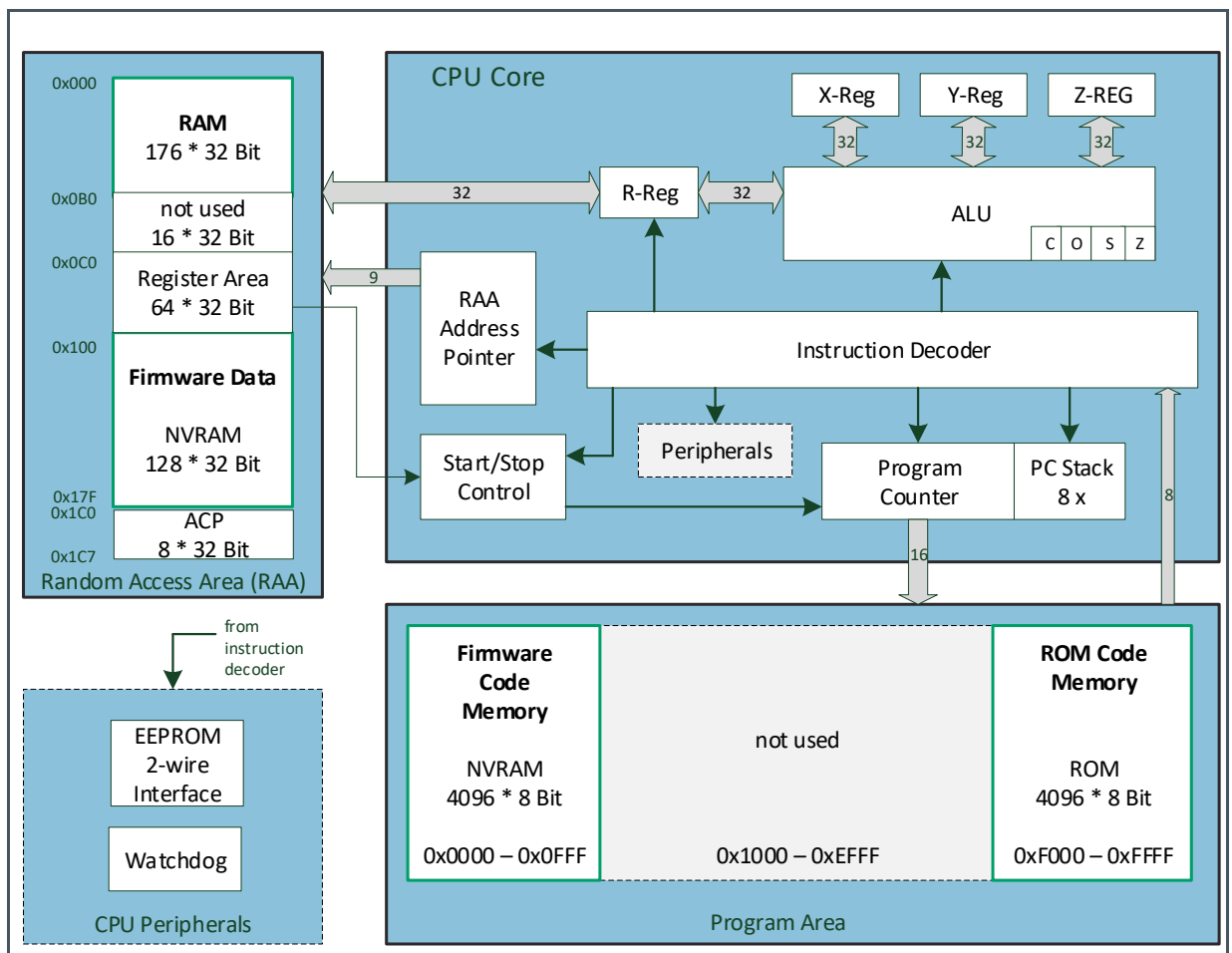
Figure 98: CPU Environment
