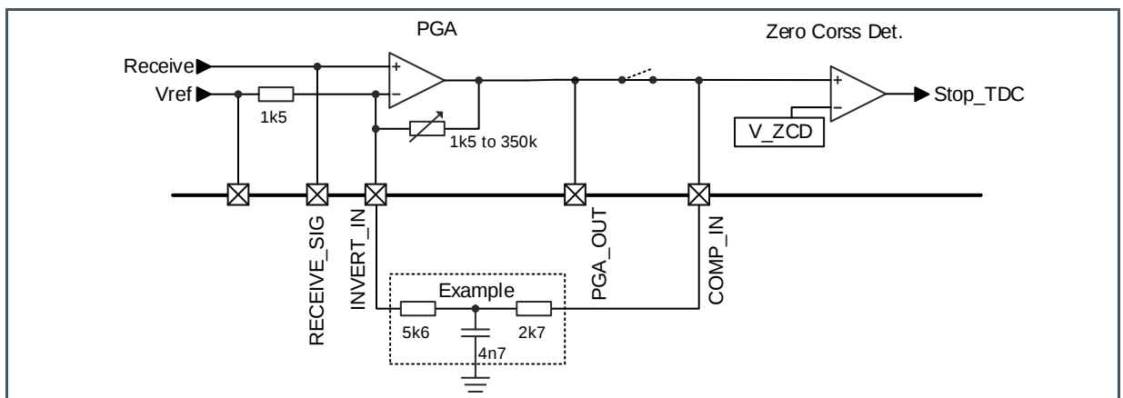
Figure 46: Wiring with PGA external Filter
