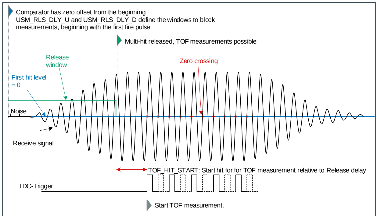
Figure 58: Release Window
