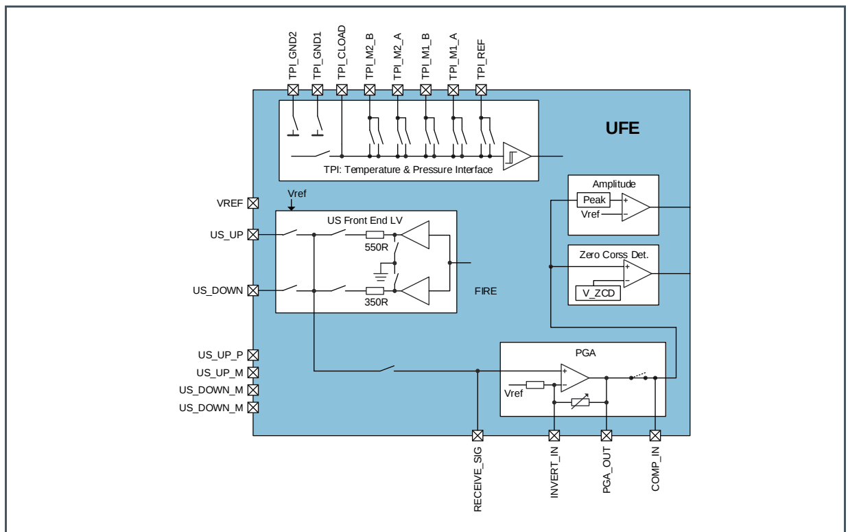
Figure 42: Ultrasonic Frontend Block
