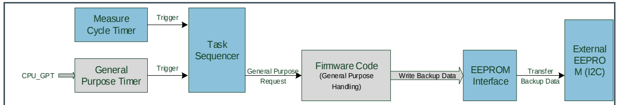
Figure 72: EEPROM Interface
