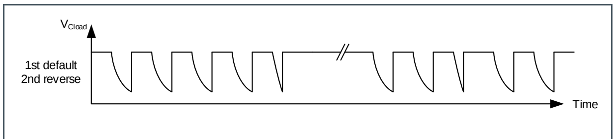
Figure 69: Voltage Cload with Internal Temperature Measurement
