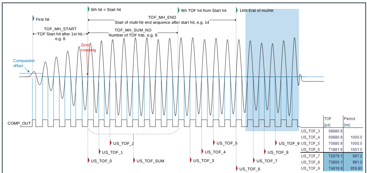
Figure 52: Receive with Split Burst, TOF_HIT_MODE = 0
