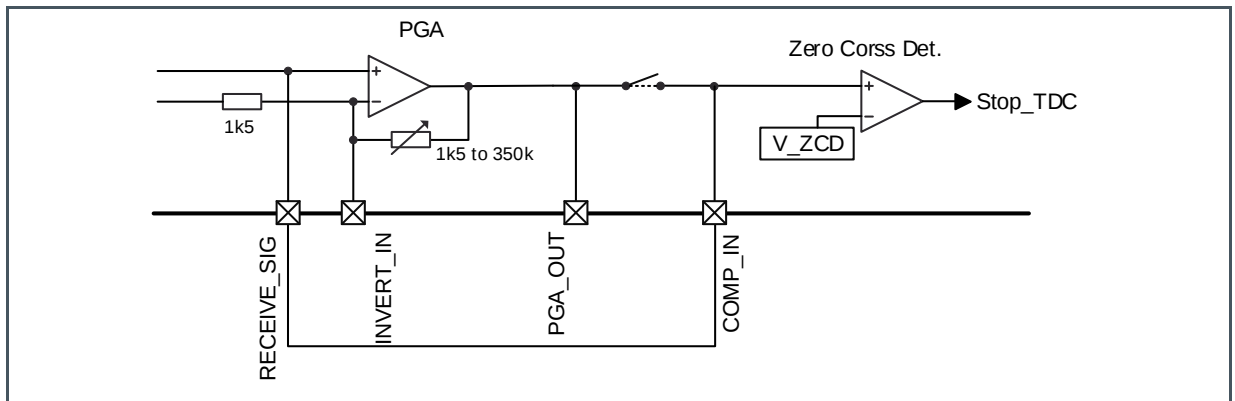
Figure 45: Wiring with PGA disabled
