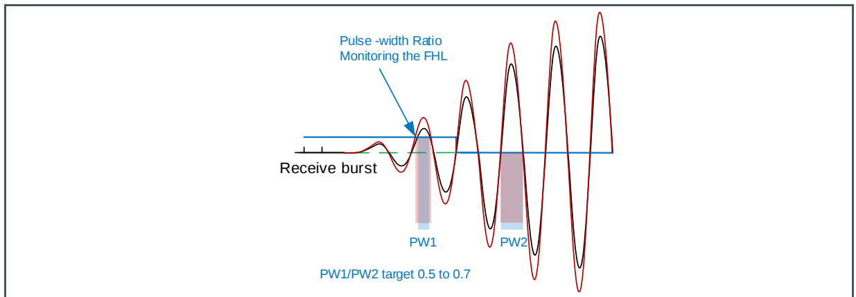
Figure 55: Pulse Width Ratio
