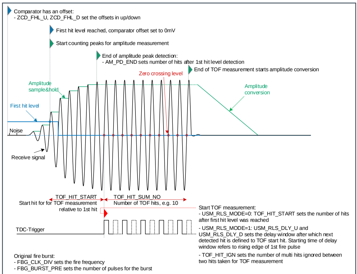
Figure 50: Time-of-flight measurement
