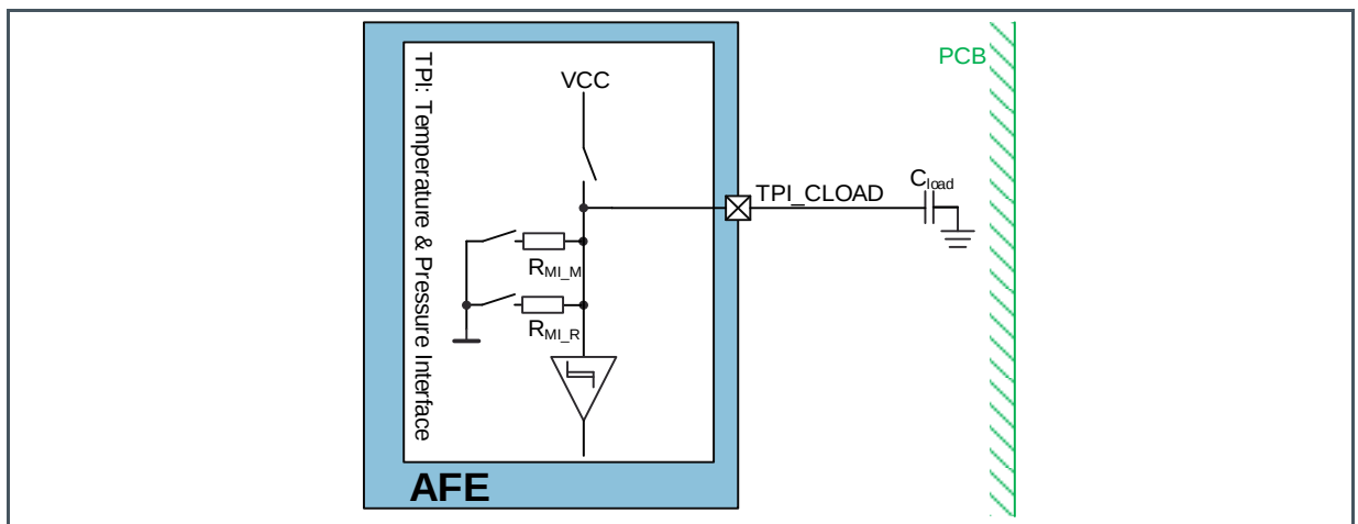
Figure 67: Internal Temperature Sensor
