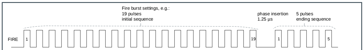
Figure 51: Split Fire Burst
