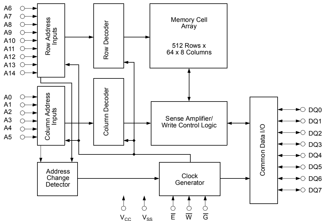
Block Diagram
