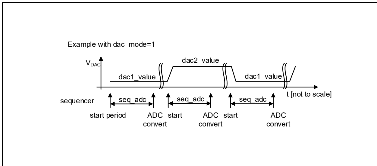
Figure 88: Electrical Analog Front End DAC Level Switching
