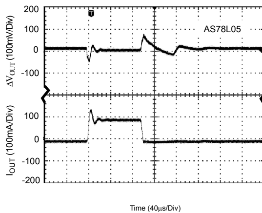
Figure 13. Load Transient
