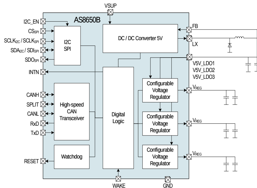
Figure 1. AS8650B Block Diagram
