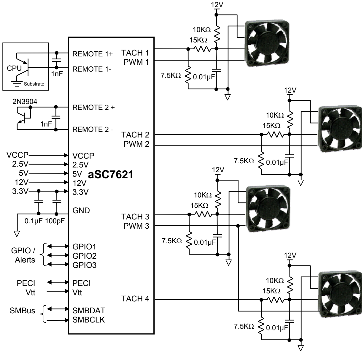
Figure 16 Application Diagram
