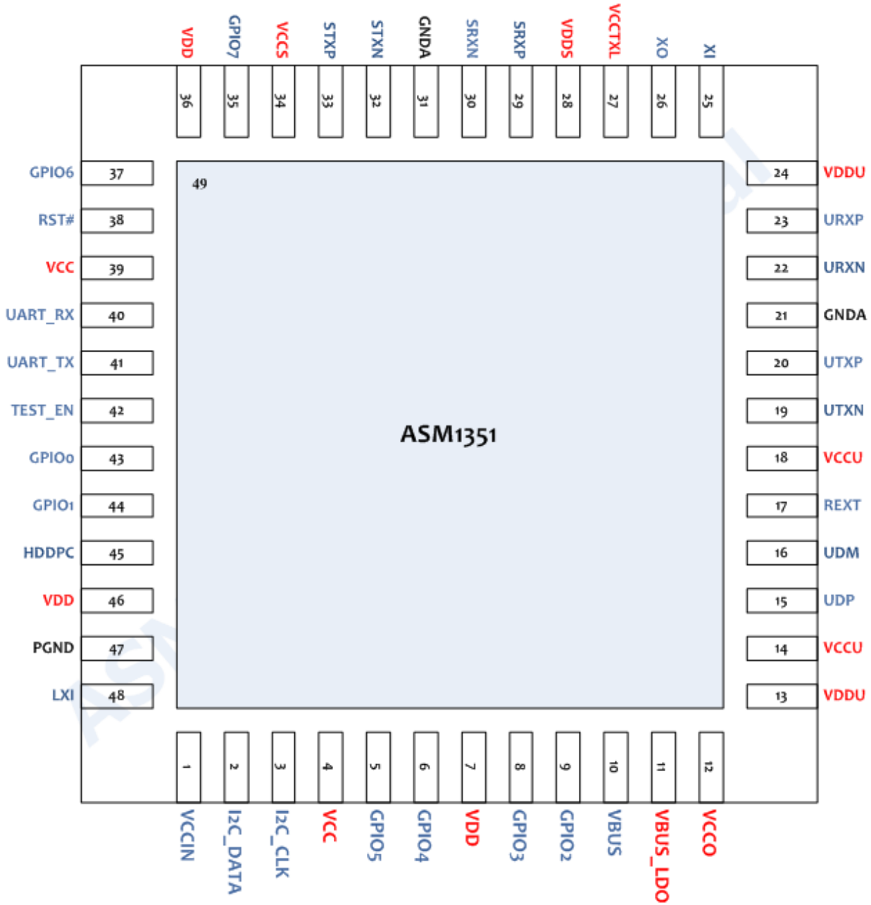
Figure 2: ASM1351 Pinout
