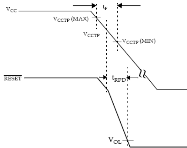
Figure 4. Timing Diagram: Power-Down
