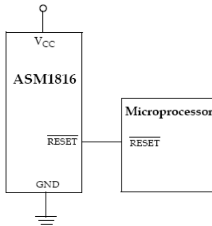
Figure 1. Typical Application
