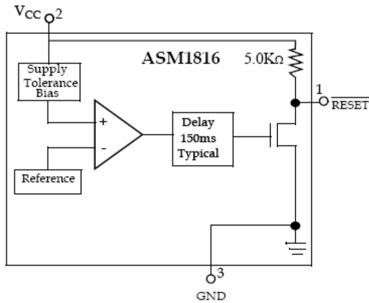
Figure 2. Block Diagram
