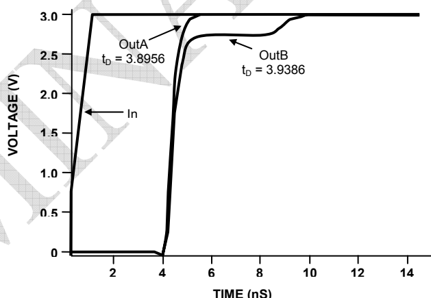
Figure 2. Single versus Dual Waveforms
