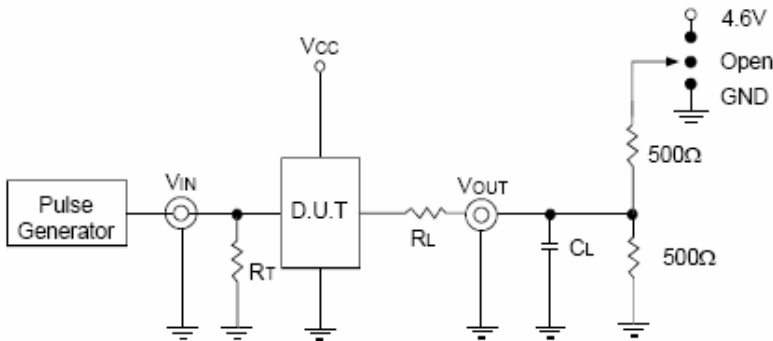
Enable and Disable Time Circuit
